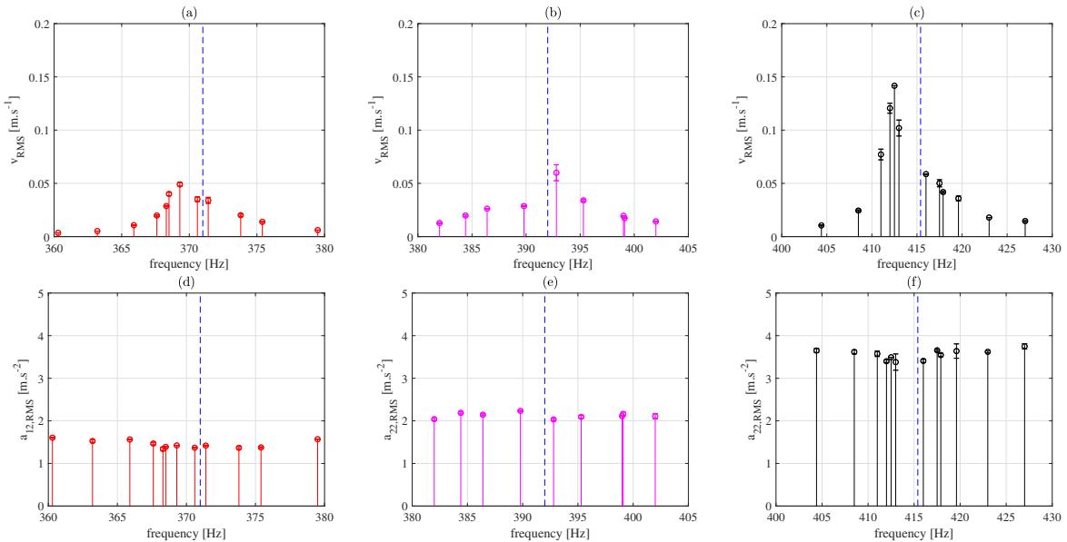
FIG. 6. RMS Velocity of the B4 (a), F4 (b) and D5 (c) S-string and RMS acceleration at point (2) on the bridge when playing the G4 (d), G#4 (e) and A4 (f) key, for f_0 in Table I.
