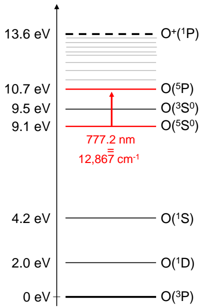
Fig. 1. Simplified distribution of O electronic energy levels with J degeneracy omitted.
