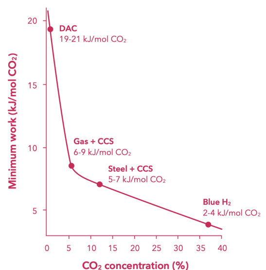
Fig. 3. Minimum energy requirements of DAC compared to those of other CCUS technologies. Adapted from Wilcox (2012) 1 .
