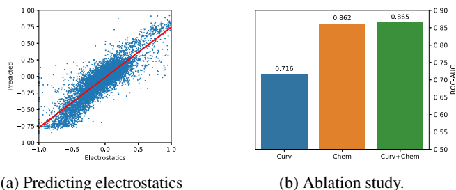
(a) Predicting electrostatics (b) Ablation study. Figure 6: Our network can compute chemical properties of the protein surface from the underlying atomic point cloud. (a) Predicted Poisson-Boltzmann electrostatic potential vs. the ground truth. Correlation cofactor r=0.83 and RMSE=0.16 . (b) Ablation study showing how chemical and geometric features affect the performance in predicting interaction sites (ROC-AUC).
