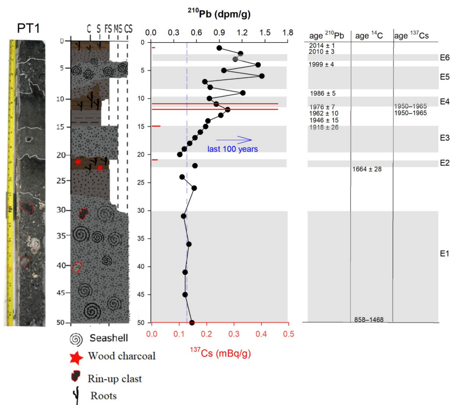
Figure 7. Lithology description, and 210 Pb (black) and 137 Cs (Red) graphic with gray bars indicating the flood and marine events identified, in correspondence with the estimated Cal BC/AD ages from radionuclide activities ( 210 Pb, 137 Cs and 14 C). The calibrated ages were obtained using the calib 8.2 program. For unit 1, an age range was obtained using three reservoir ages according to the values reported for this area (see Table 1).
