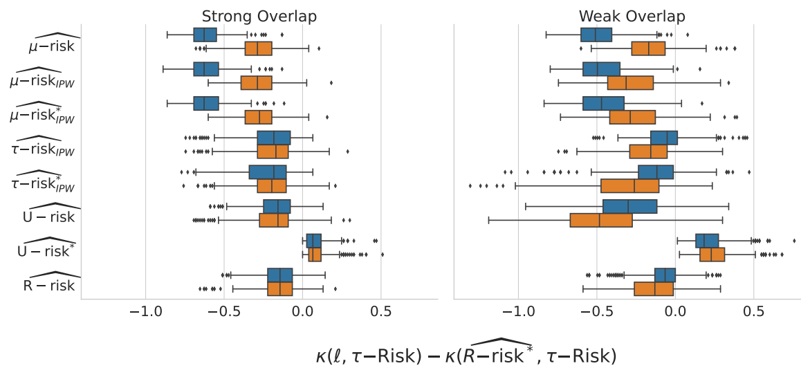
Figure 17. Results are similar between the Shared nuisances/candidate set and the Separated nuisances set procedure. The experience has not been run on the full metrics for Caussim due to computation costs.
