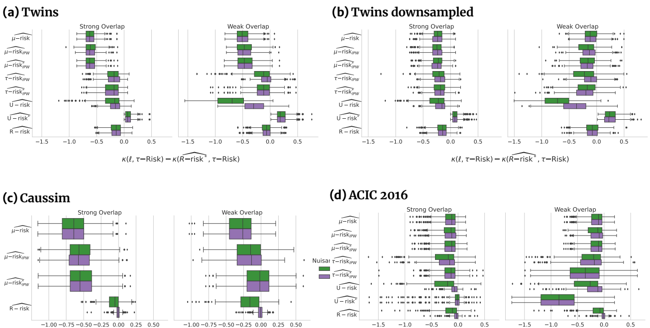
Figure 19. Learning the nuisances with stacked models (linear and gradient boosting) is important for successful model selection with R -risk. For Twins dataset, there is no improvement for stacked models compared to linear models because of the linearity of the propensity model.
