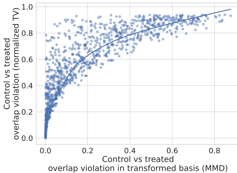
Figure 11. Good correlation between overlap measured as normalized Total Variation and Maximum Mean Discrepancy (200 sampled Caussim datasets)
