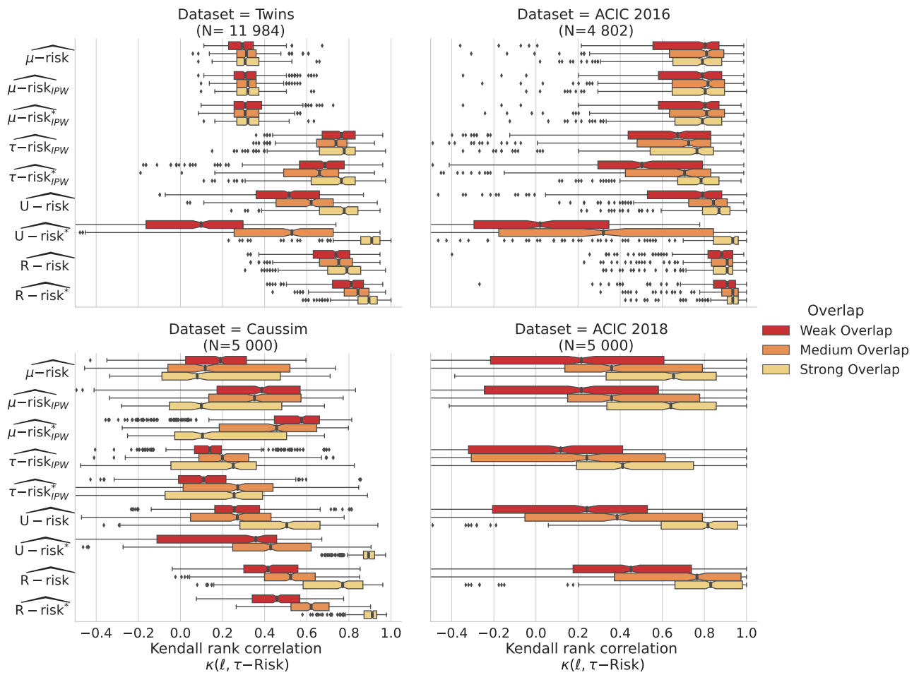
Figure 18. Low population overlap hinders causal model selection for all metrics: Kendall's \tau agreement with \tau -risk. Strong, medium and Weak overlap correspond to the tertiles of the overlap distribution measured with Normalized Total Variation eq. 17.
