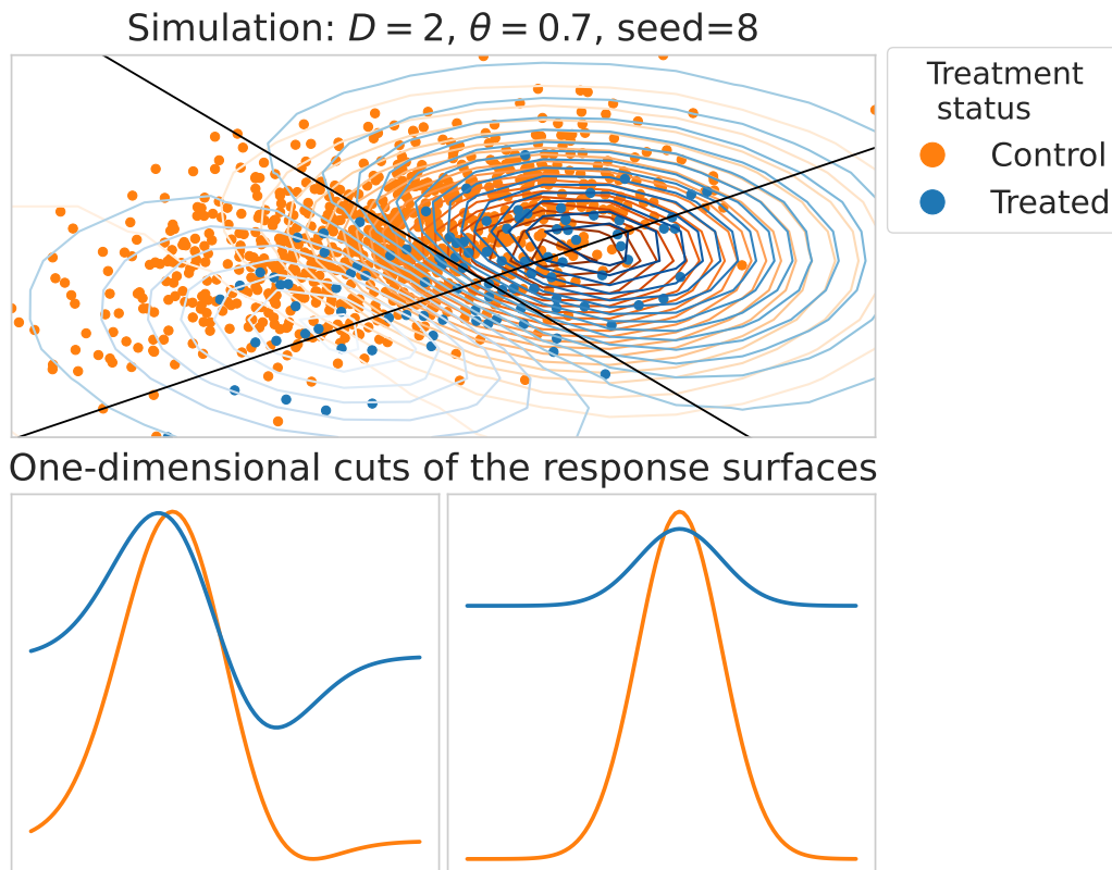
Figure 13. Example of the simulation setup in the input space with two knots –ie. basis functions. The top panel shows the observations in feature space, while the bottom panel displays the two response surfaces on a 1D cut along the black lines drawn on the top panel.
