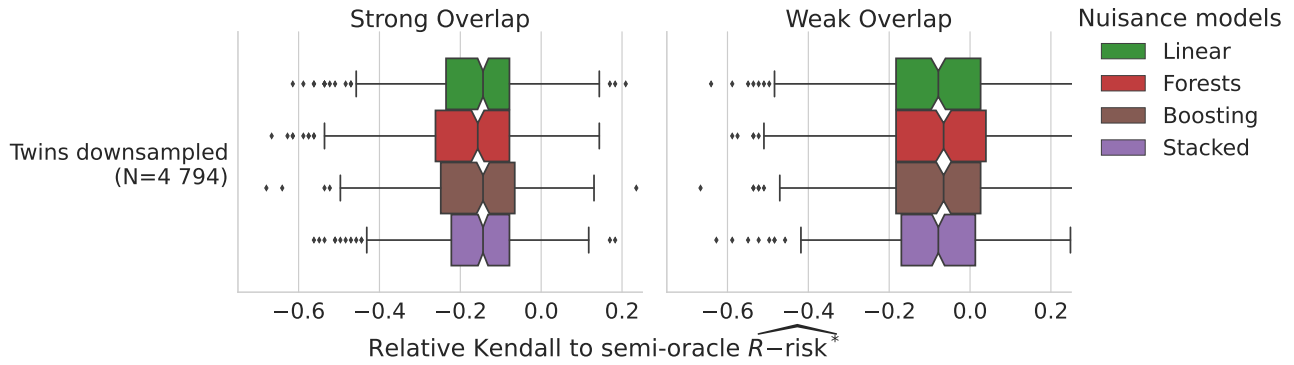
Figure 20. Flexible models are performant in recovering nuisances in the downsampled Twins dataset. The propensity score is linear in this setup, making it particularly challenging for flexible models compared to linear methods.
