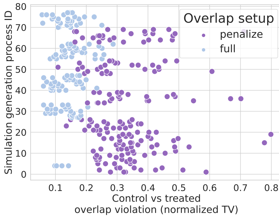
Figure 10. NTV recovers well the overlap settings described in the ACIC paper [45]
