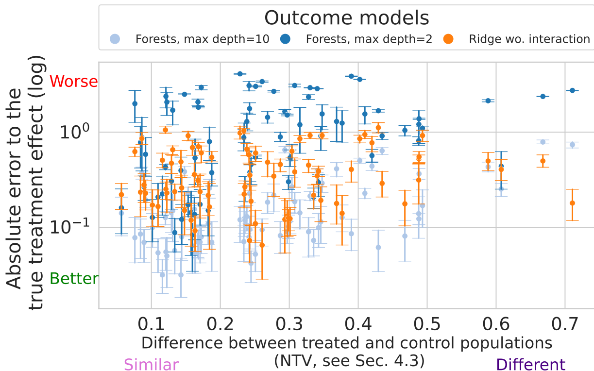
Figure 8. Different outcome models lead to different estimation errors on the Average Treatment Effects, on 77 classic simulations with known true causal effect [45]. The different models are ridge regression and random forests with different hyper-parameters (details A.1). The different configurations are plotted as a function of increasing difference between treated and untreated population –see subsection . There is no systematic best performer; data-driven model selection is important.
