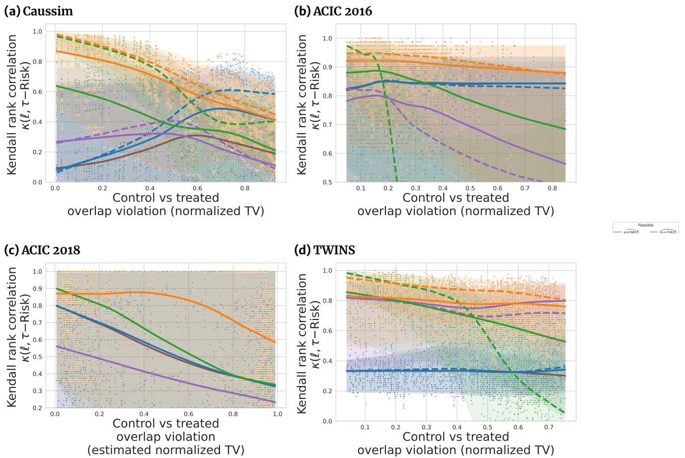
Figure 15. Agreement with \tau -risk ranking of methods function of overlap violation. The lines represent medians, estimated with a lowess. The transparent bands denote the 5% and 95% confidence intervals.
