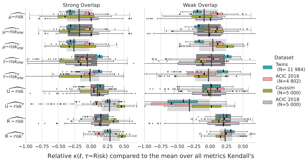
Figure 14. The R -risk is the best metric on average: Relative Kendall's \tau agreement with \tau -risk. Strong and Weak overlap correspond to the first and last tertiles of the overlap distribution measured with Normalized Total Variation eq. 17.
