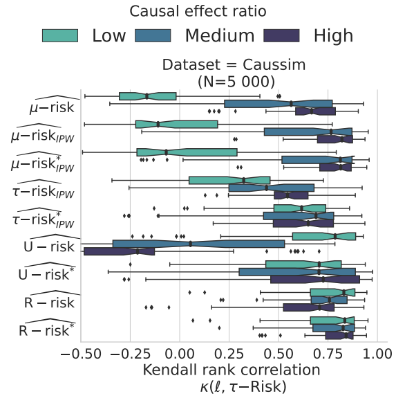
Figure 7. R -risk is robust to a wide range of effect ratio: Kendall's \tau agreement with \tau -risk. Strong, medium and Weak Causal effect ratio are the tertiles of the absolute ratio causal effect to baseline response, \Delta_\mu : Low [0.04; 2.86], Medium [2.86; 16.65], High [16.65; 206.53]. Appendix A.9 details this simulation.
