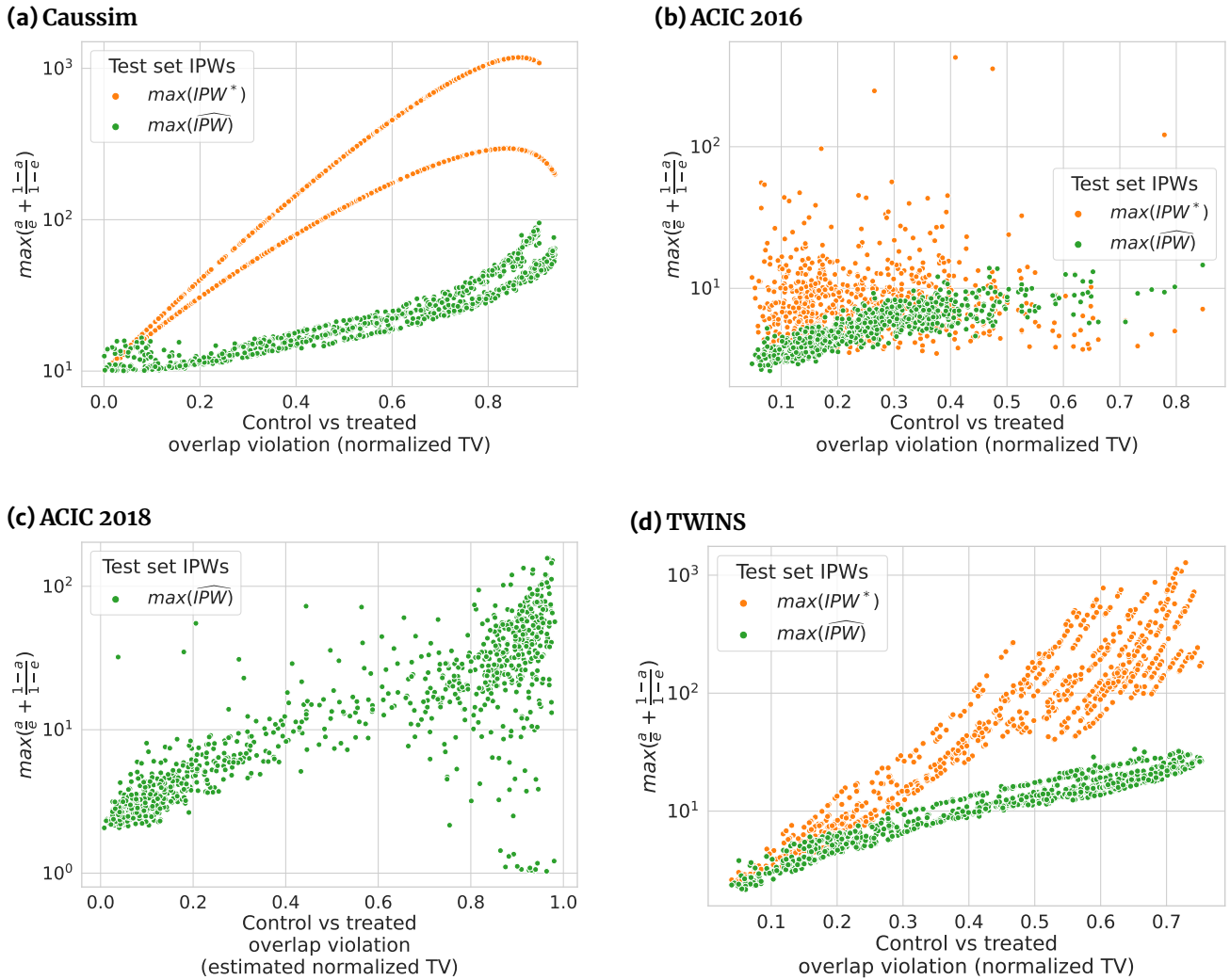
Figure 12. Maximal value of Inverse Propensity Weights increases exponentially with the overlap as measure by Normalized Total Variation.
