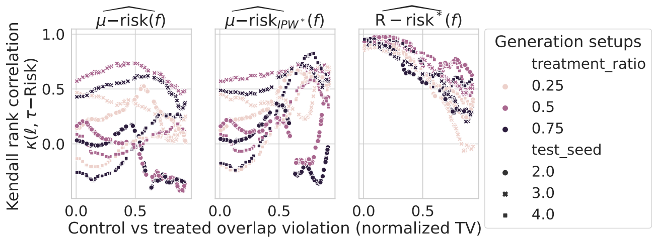
Figure 21. Kendall correlation coefficients for each causal metric. Each (color, shape) pair indicates a different (treatment ratio, seed) of the generation process.
