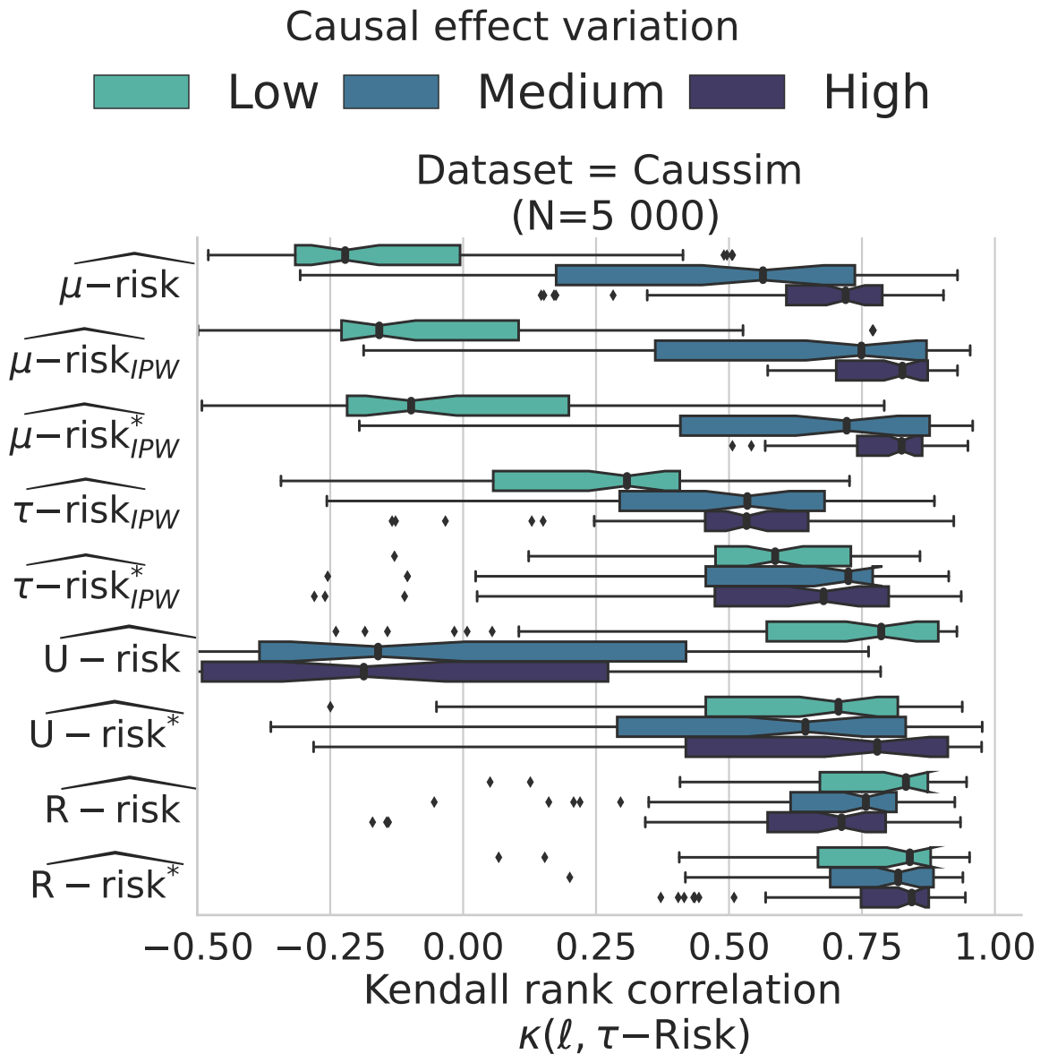
Figure 23. R-risk is robust to a wide range of effect variance: Kendall's \tau agreement with \tau -risk. Strong, medium and Weak Causal effect variance are the tertiles of the ratio of causal effect variance to the mean outcome variance: Low [0; 0.04], Medium [0.04; 1.04], High [1.04; 11.08].
