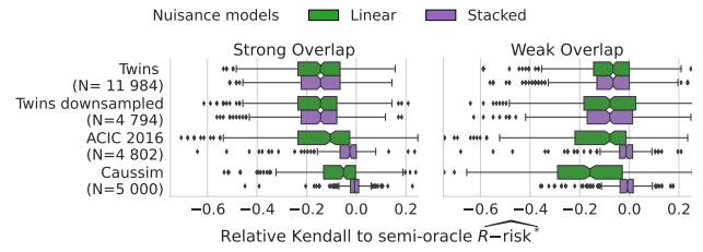
Figure 6. Stacked models are good overall estimators of the nuisances: Results are shown only for the R -risk; Figure 19 details every metrics. For Twins, where the true propensity model is linear, stacked and linear estimations of the nuisances performs equivalently, even for a downsampled version ( N=4,794 ).
