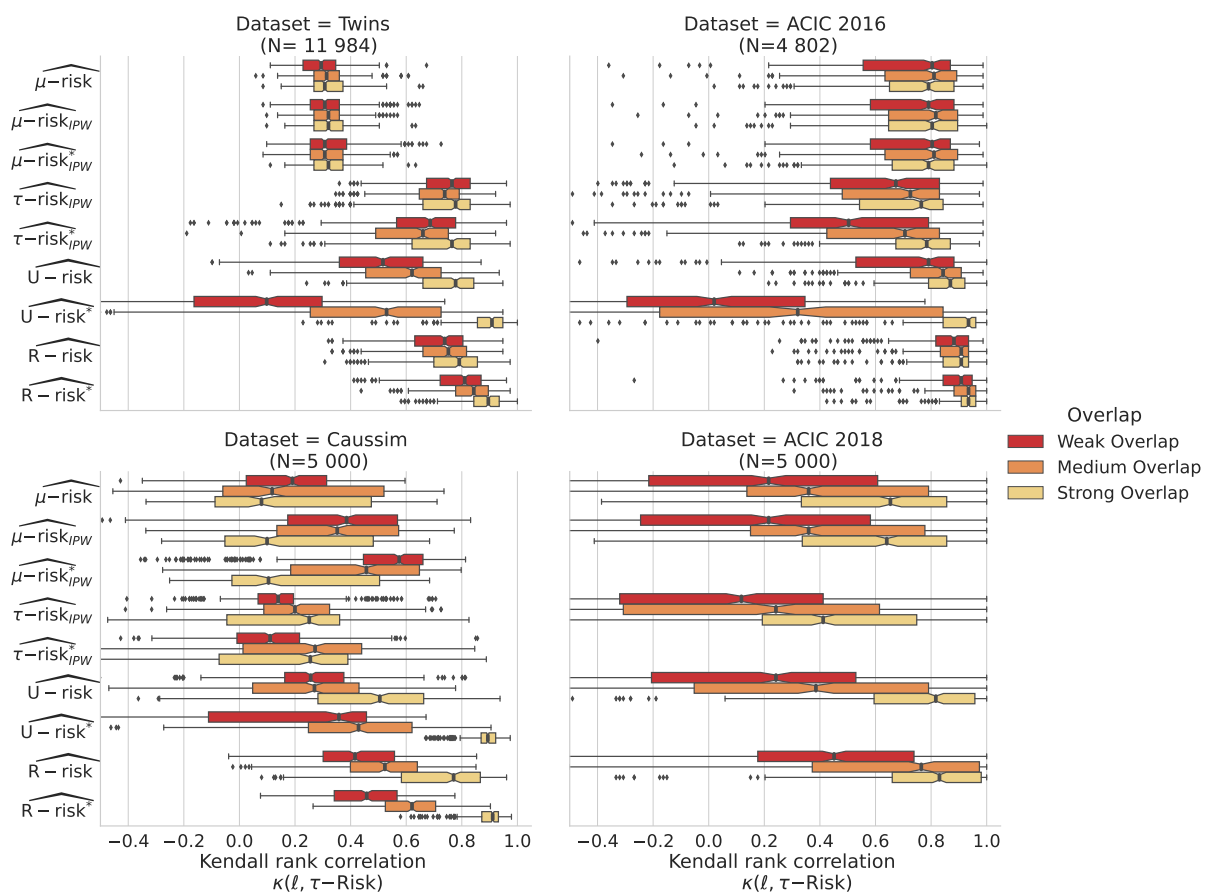
Figure 17: Low population overlap hinders causal model selection for all metrics: Kendall's \tau agreement with \tau\text{-risk} . Strong, medium and Weak overlap correspond to the tertiles of the overlap distribution measured with Normalized Total Variation eq. 16.
