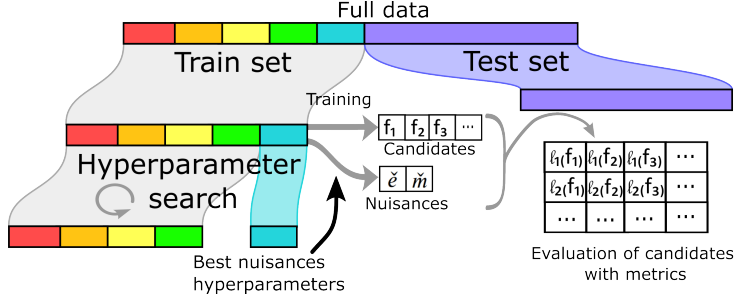
Figure 2: Estimation procedure for causal model selection.
