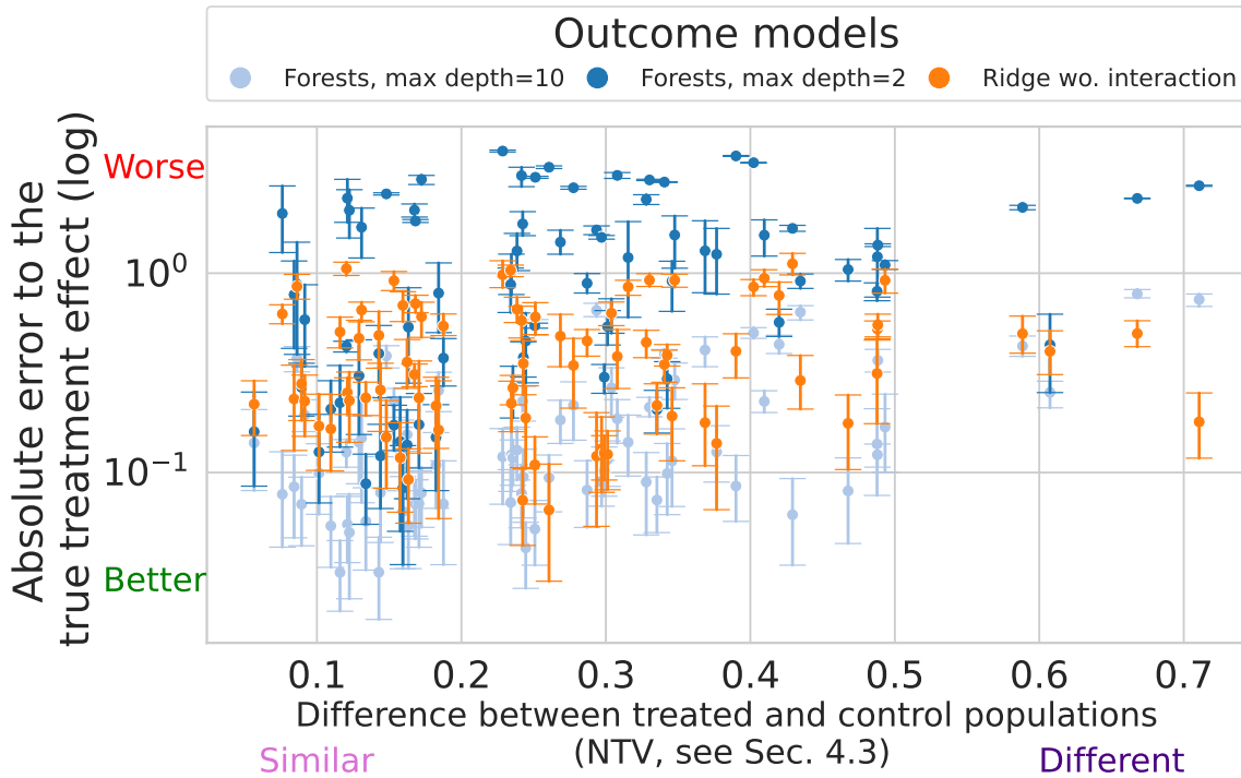
Figure 7: Different outcome models lead to different estimation errors on the Average Treatment Effects, on 77 classic simulations with known true causal effect 18 . The different models are ridge regression and random forests with different hyper-parameters (details A). The different configurations are plotted as a function of increasing difference between treated and untreated population –see section . There is no systematic best performer; data-driven model selection is important.
