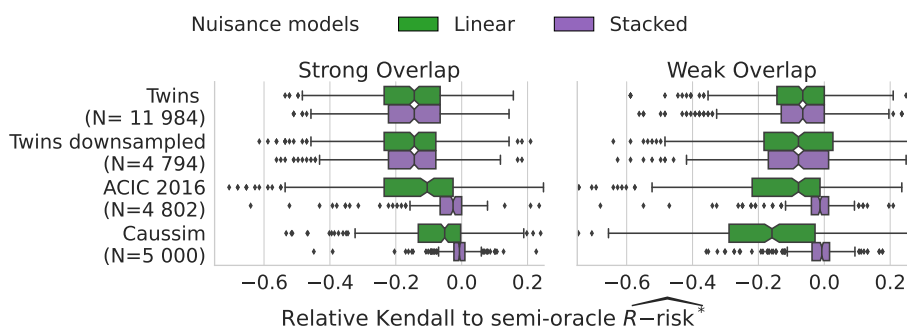
Figure 6: Stacked models are good overall estimators of the nuisances: Results are shown only for the R-risk; Figure 18 details every metrics. For Twins, where the true propensity model is linear, stacked and linear estimations of the nuisances performs equivalently, even for a downsampled version (N=4,794).
