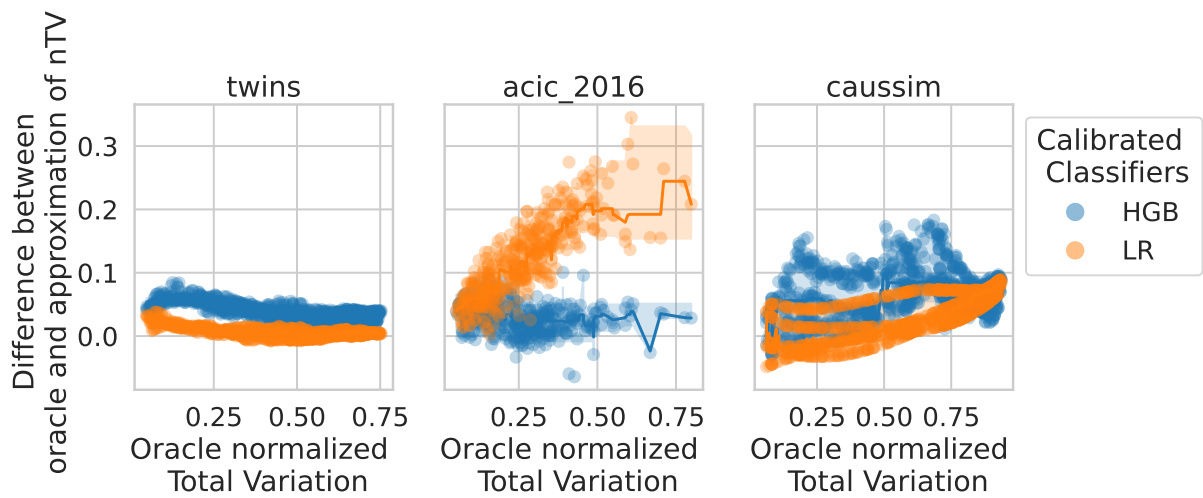
Figure 8: a) Without calibration, estimation of NTV is not trivial even for boosting models. b) Calibrated classifiers are able to recover the true Normalized Total Variation for all datasets where it is available.
