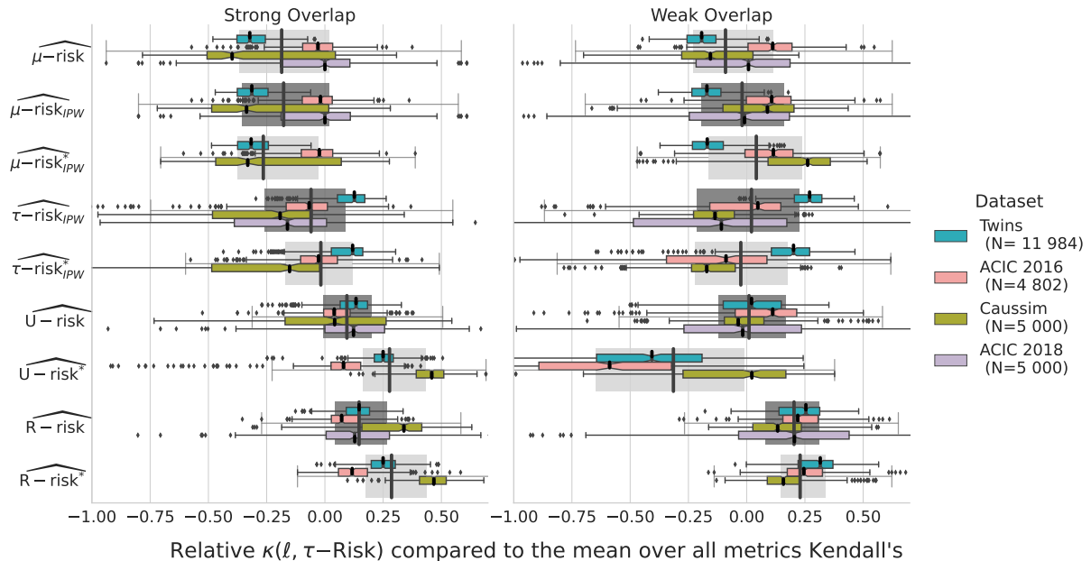
Figure 13: The R -risk is the best metric: Relative Kendall's \tau agreement with \tau -risk. Strong and Weak overlap correspond to the first and last tertiles of the overlap distribution measured with Normalized Total Variation eq. 16.
