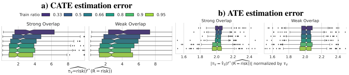
Figure 21: a) For CATE, a train/test ratio of 0.9/0.1 appears a good trade-off. b) For ATE, there is a small signal pointing also to 0.9/0.1 ( K=10 ). for ATE. Experiences on 10 replications of all 78 instances of the ACIC 2016 data.
