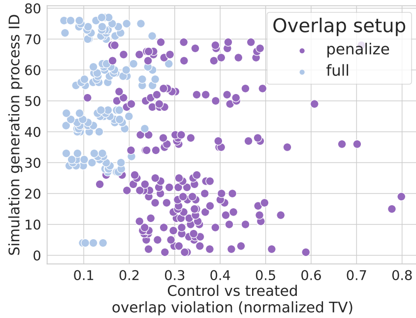
Figure 9: NTV recovers well the overlap settings described in the ACIC paper 18
