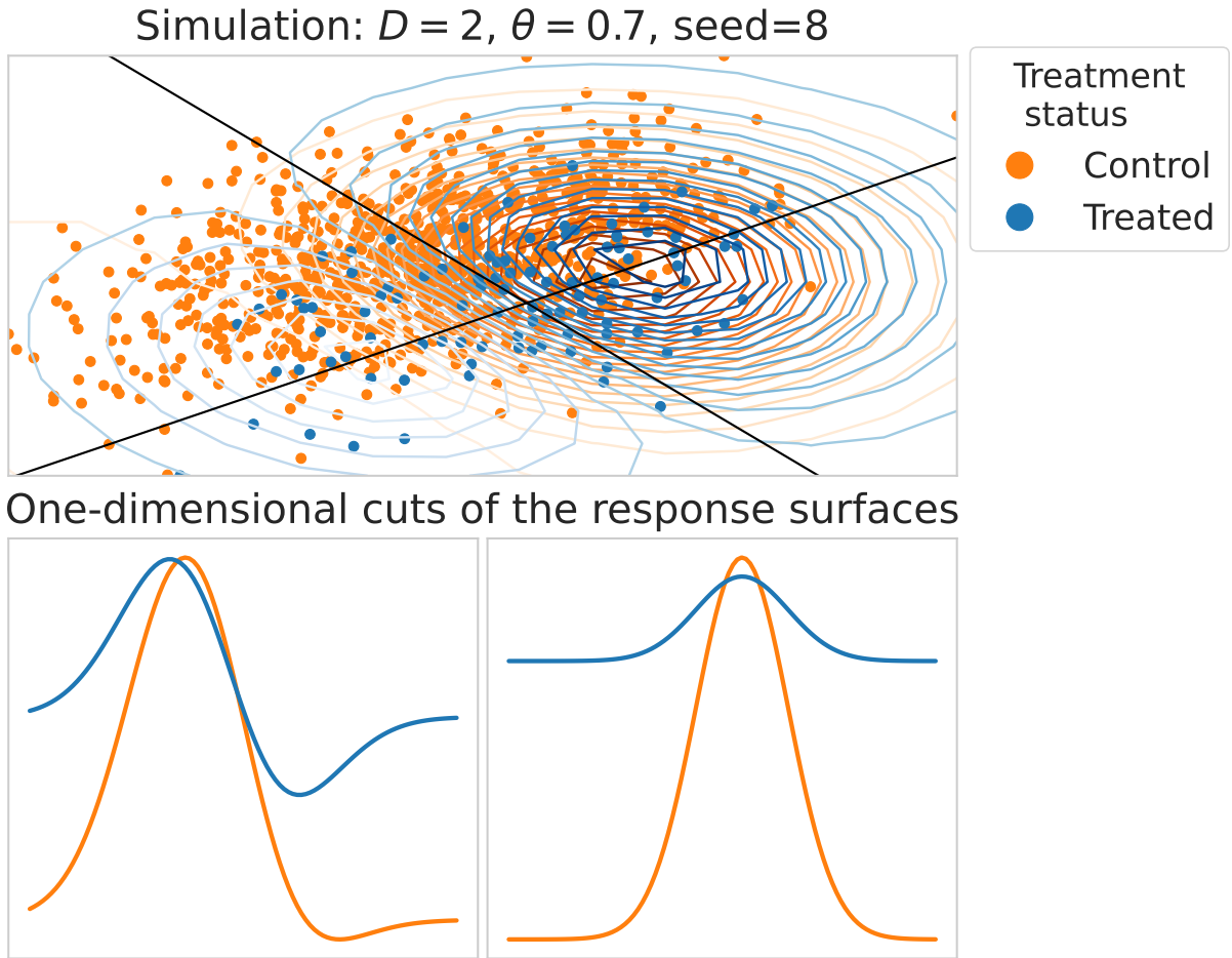
Figure 12: Example of the simulation setup in the input space with two knots –ie. basis functions. The top panel shows the observations in feature space, while the bottom panel displays the two response surfaces on a 1D cut along the black lines drawn on the top panel.
