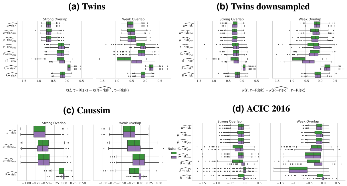
Figure 18: Learning the nuisances with stacked models (linear and gradient boosting) is important for successful model selection with R-risk. For Twins dataset, there is no improvement for stacked models compared to linear models because of the linearity of the propensity model.
