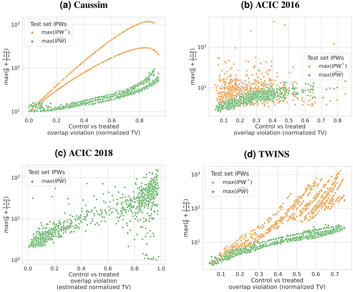
Figure 11: Maximal value of Inverse Propensity Weights increases exponentially with the overlap as measure by Normalized Total Variation.
