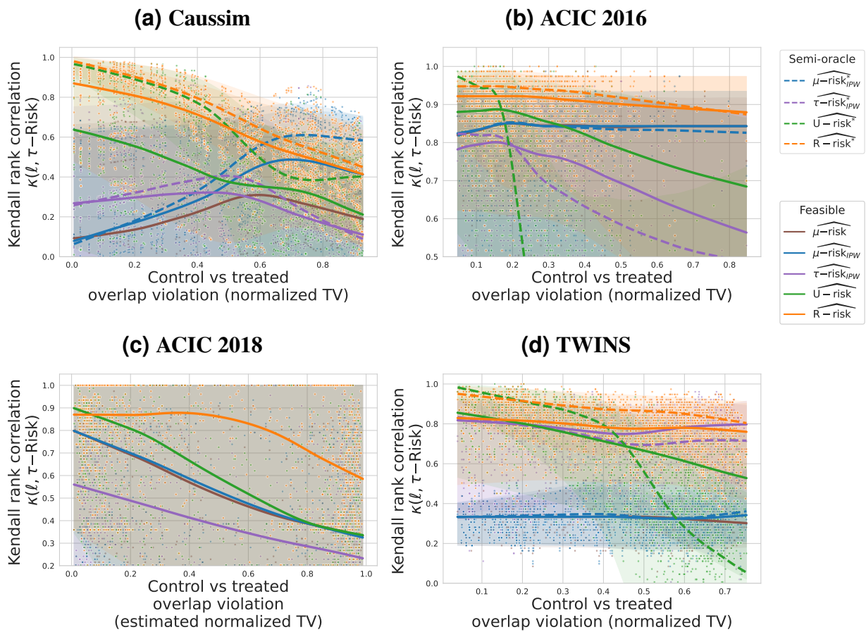
Figure 14: Agreement with \tau -risk ranking of methods function of overlap violation. The lines represent medians, estimated with a lowess. The transparent bands denote the 5% and 95% confidence intervals.
