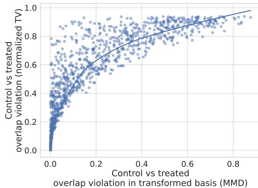
Figure 10: Good correlation between overlap measured as normalized Total Variation and Maximum Mean Discrepancy (200 sampled Caussim datasets)
