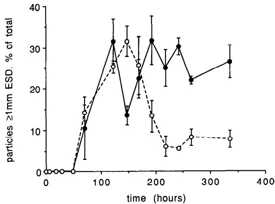
Fig. 2. Development of the abundance of aggregates \geq 1 -mm ESD expressed as percent of total particles present in natural seawater incubated in rotating cylindrical tanks. In three tanks, the concentration of VLPs was increased 2.3-fold (●) and compared to untreated natural seawater (○). Values are means of triplicate incubations.
