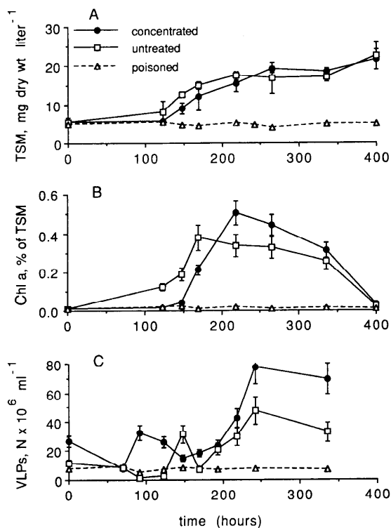
Fig. 1. Effect of adding the virus-rich 2–200-nm size fraction concentrated from seawater and of cyanide poisoning on the development of total suspended matter, the percentage of Chl a in TSM, and the change in abundance of viruslike particles (VLPs). Values are means of duplicate (poisoned treatments) or triplicate incubations; viruses were counted in one poisoned, two enriched, and two untreated cultures. Vertical bars indicate mean deviations.
