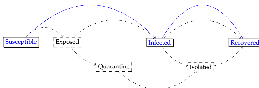
Figure 1. The SIR model and extensions. The basic three compartments are shown in blue and connected by plain lines. A Possible extension is illustrated through three further compartments connected with dashed lines.
