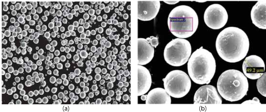
Figure 2. Ti-6Al-4V spherical powder morphology: (a) 100×; (b) 400×.
