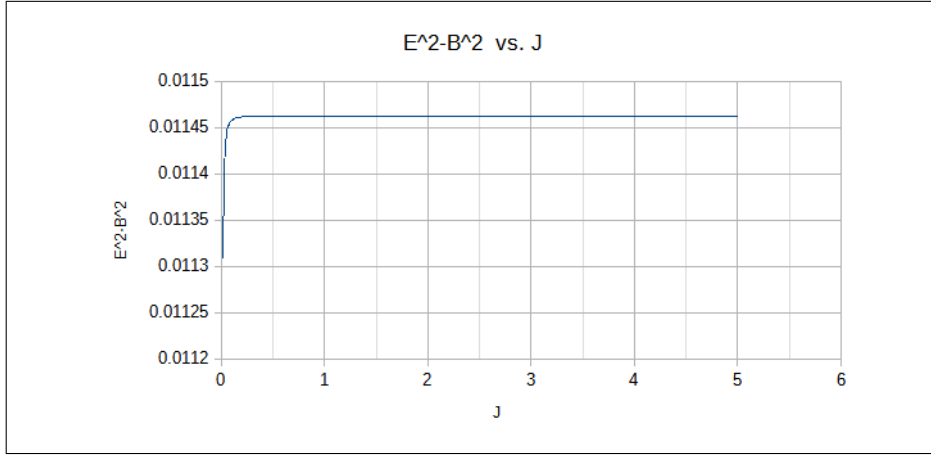
Figure 4: Volume integral of \mathbf{E}^2 - \mathbf{B}^2
