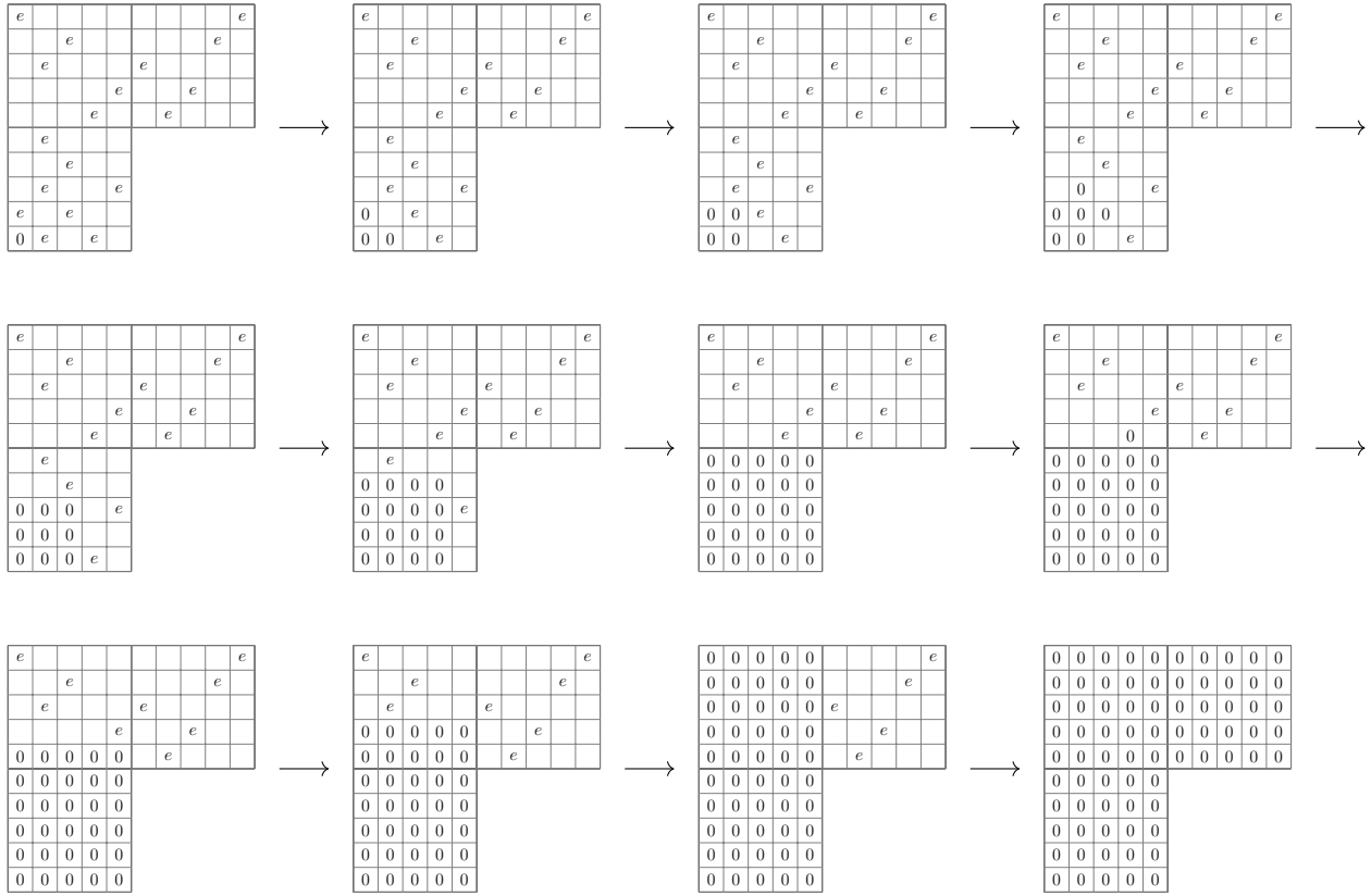
FIGURE 5.1. First steps of propagating the empty cluster. 0 represents an empty site, otherwise the state is the initial one. e stands for an easy site.
