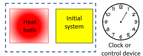
FIG. 2. Schematic of the autonomous quantum devices we focus on: a nonautonomous thermal machine complemented by a quantum clock. The system in the dotted-line box is the same as in Fig. 1(b). It depicts the standard systems involved in the resource-theoretic approach to thermodynamics. If no other systems are involved, its dynamics are described by a time-dependent Hamiltonian. If one includes an additional quantum system whose state changes in a predictable fashion with the passing of time, i.e., a clock, then it can turn on and off interaction terms at specific times, leading to an autonomous implementation of the resource-theoretic approach to thermodynamics. Hence, we use a clock as a control device.
