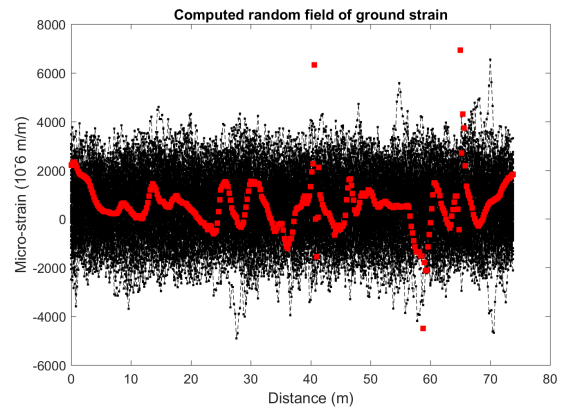
Figure 7: Ground strain measurements for series LSO (in red dotted line) and computed random field of ground strain (100 simulations in black dotted line) below the pipeline for June 2017.
