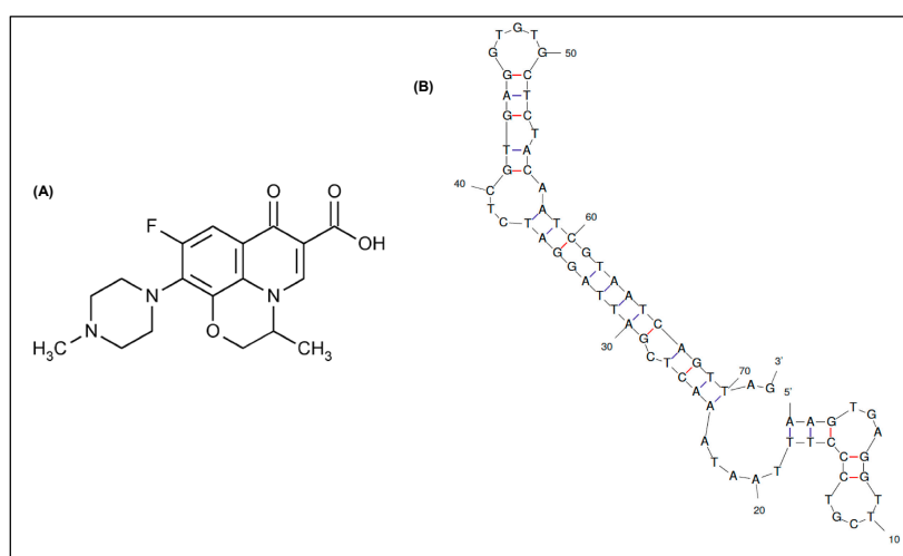
Figure 1. (A) Chemical structure of ofloxacin. (B) 2-D structure of the truncated DNA aptamer modeled by Mfold web server [27] ( \Delta G = -24.36\text{ kcal/mol} ).
