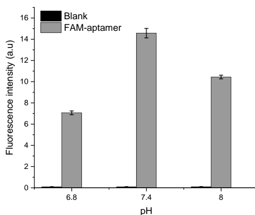
Figure 6. pH optimization based on the FAM-APT fluorescence intensity at 0.25 \mu\text{M} .
