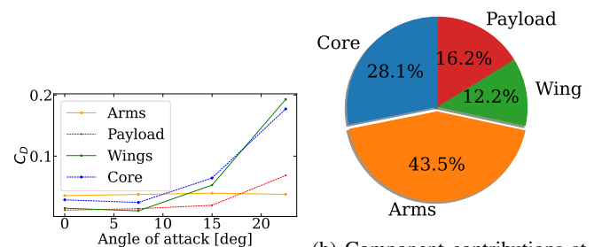
(a) Drag with respect to \alpha (b) Component contributions at \alpha of 7.5°
