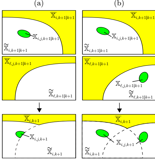
Fig. 3. Set estimates evaluated by UAVs i and \ell before communication (two top subfigures) and after communication and update (bottom subfigures); (a) \bar{X}_{i,j,k+1} is smaller than \bar{X}_{i,j,k+1|k+1} since some subsets of \bar{X}_{i,j,k+1|k+1} have been proved by UAV \ell not to contain a target; (b) \bar{X}_{i,j,k+1} is larger than \bar{X}_{i,j,k+1|k+1} , since both UAVs have to account for the two different hypotheses on the state estimate of target j .
