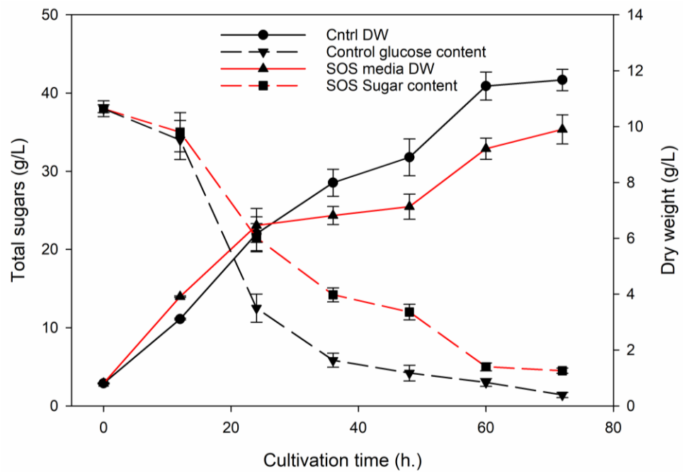
Figure 5. Growth curves and sugar consumption over time for A. mangrovei using the SOS optimized media compared to their relative control at the same C/N ratio using glucose. Values are reported as mean \pm SD.
