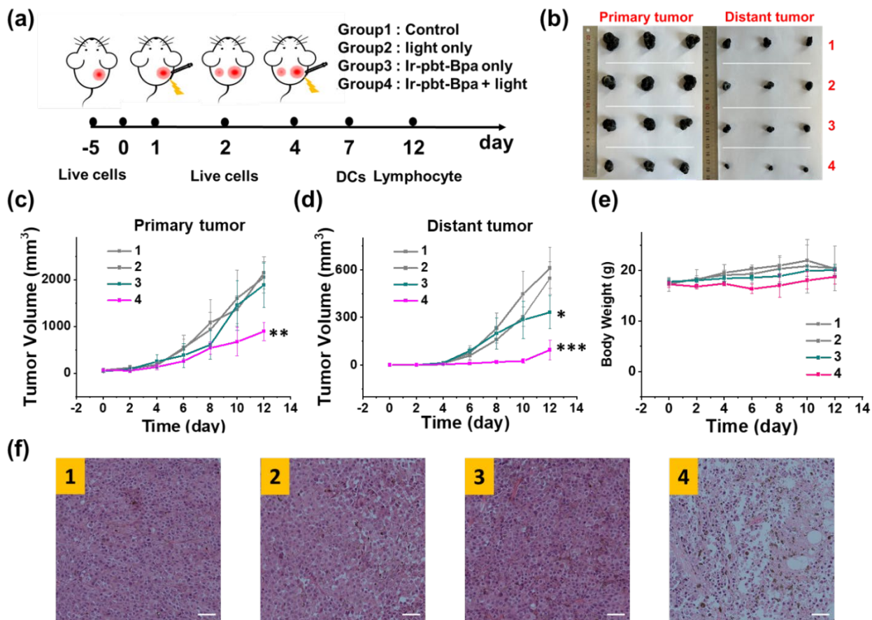
Fig. 5 The treatment of mice models. Evaluation of the treatment of mice models with primary and distant B16F10 mice melanoma tumors upon intratumor injection of Ir-pbt-Bpa (3 mg/kg) into the primary tumor and exposure to two-photon irradiation (750 nm, 50 mW, 5 min). (a) Schematic timeline of the treatment. (b) Photographs of the collected tumors 12 days after the treatment. (c) Change in the tumor volume of the primary tumor upon treatment. (d) Change in the tumor volume of the secondary tumor upon treatment. (e) Change of the weight of the animal models. (f) Histological examination of the secondary tumor with a hematoxylin and eosin stain 12 days after the treatment. 1) Control; 2) light only; 3) Ir-pbt-Bpa only; 4) Ir-pbt-Bpa + light. *** P < 0.001 , ** P < 0.01 and * P < 0.05 , in comparison to control.
