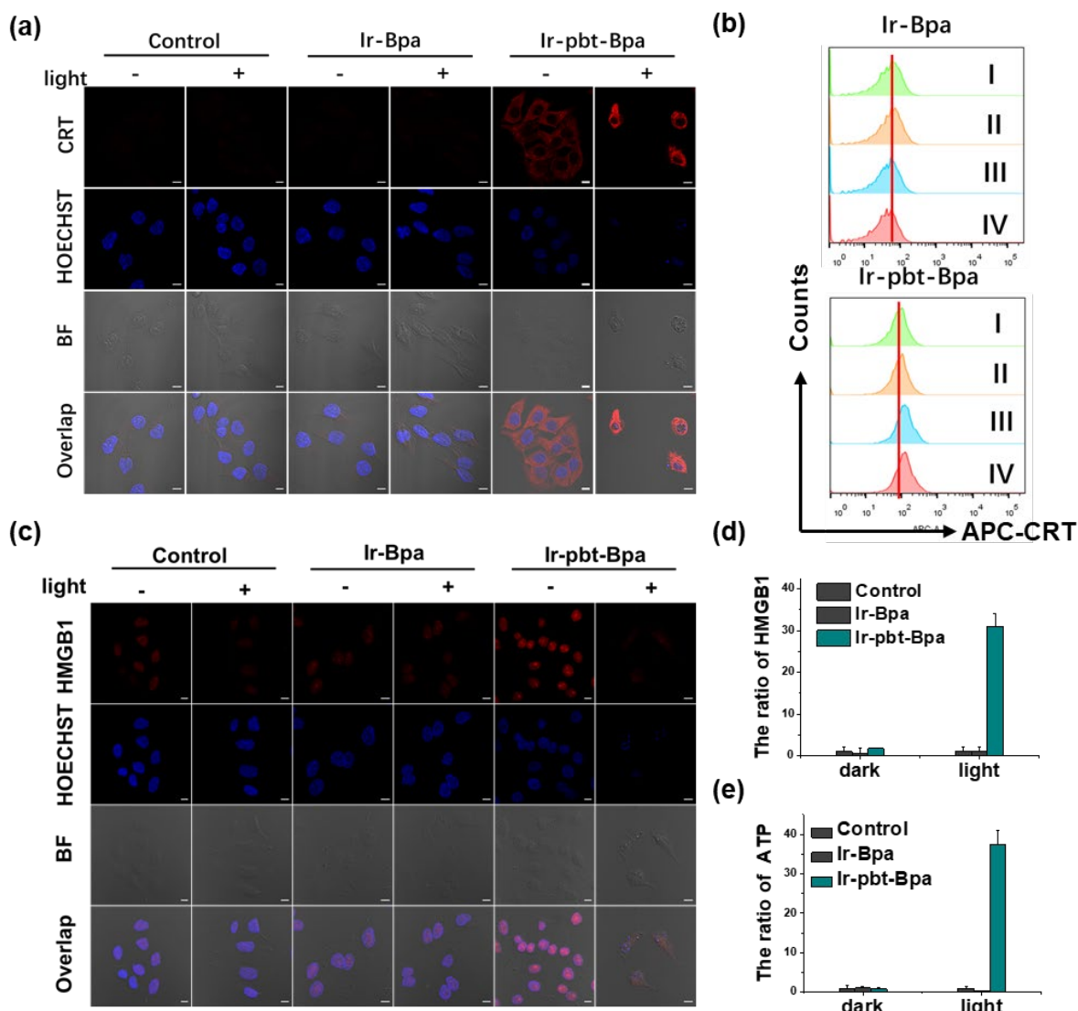
Fig. 3 Evaluation for hallmarks of ICD in A375 cells. Evaluation for hallmarks of ICD in A375 cells upon treatment with Ir-Bpa (1 \mu M) and Ir-pbt-Bpa (1 \mu M) in the dark or upon irradiation (405 nm LED, 0.75 J/cm 2 ). (a) Immunofluorescence confocal laser scanning microscopy stained with a calreticulin-specific antibody. Scale bar: 10 \mu m. (b) Flow cytometry spectrum to investigate the translocation of calreticulin. (I): Cells were kept in the dark; (II): Cells were exposed to irradiation (405 nm LED, 0.75 J/cm 2 ); (III): Cells were incubated with Ir-pbt-Bpa (1 \mu M) for 4 h in the dark, (IV): Cells were incubated with Ir-pbt-Bpa (1 \mu M) for 4 h and exposed to irradiation (405 nm LED, 0.75 J/cm 2 ). (c) Immunofluorescence confocal laser scanning microscopy stained with a nuclear high-mobility group box 1 protein-specific antibody. Scale bar: 10 \mu m. (d) Release of nuclear high-mobility group box 1 protein into the cell culture supernatant. e Release of adenosine triphosphate into the cell culture supernatant.
