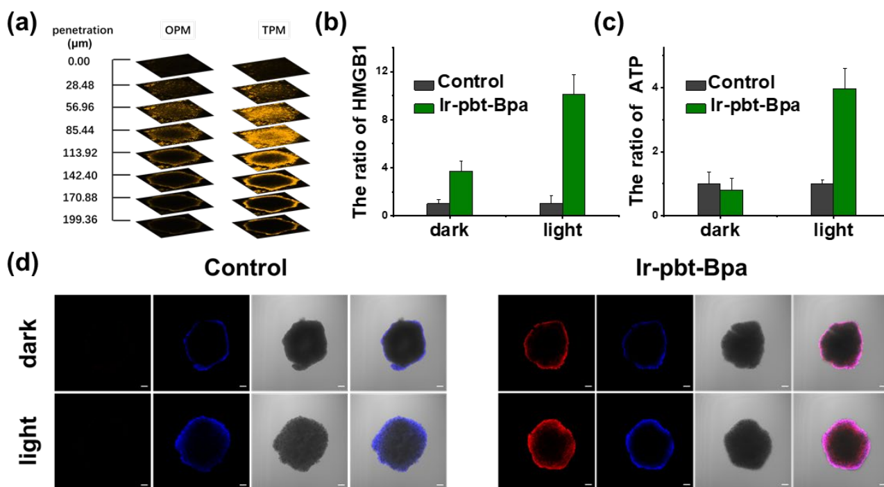
Fig. 4 Evaluation for hallmarks of ICD in A375 MCTS. Evaluation for hallmarks of ICD in A375 MCTS upon treatment with Ir-pbt-Bpa (5 μM) in the dark or upon two-photon irradiation (750 nm, 50 mW, 5 min). (a) One- (OPM) and two-photon (TPM) excited z-stack confocal laser scanning microscopy upon incubation for 12 h. (b) Release of nuclear high-mobility group box 1 protein into the cell culture supernatant. (c) Release of adenosine triphosphate into the cell culture supernatant. (d) Immunofluorescence confocal laser scanning microscopy stained with a nuclear high-mobility group box 1 protein-specific antibody (red) and 4',6-Diamidino-2-phenylindol (blue). Scale bar: 100 μm
