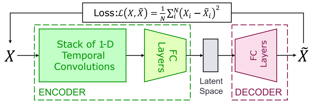
Figure 5. Convolutional Autoencoders Architecture for the processing of sequential data, such as SAR time series.
