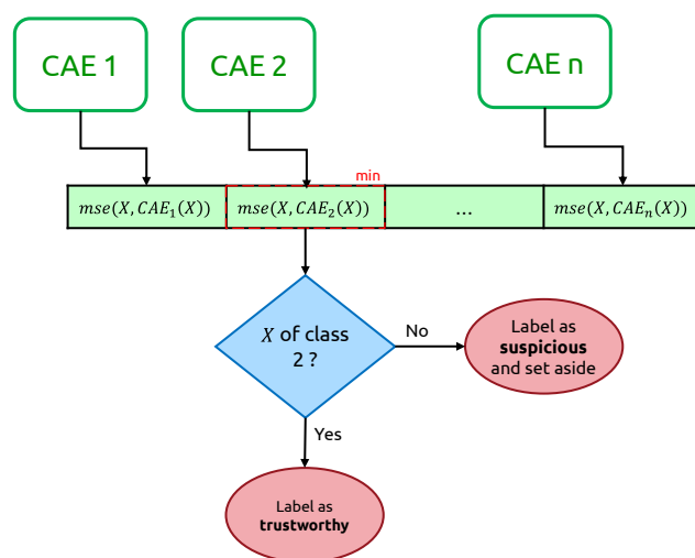
Figure 8. Illustration of a vector of Mean-Squared errors, used to identify suspicious and non-suspicious time series.
