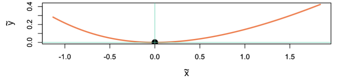
Figure 5: The representation in the new coordinate system \tilde{x}, \tilde{y} of the curve defined by function g(x) in the considered example. The new coordinate axis \tilde{x} aligns effectively with the curve, especially in the neighborhood around the reference point P .
