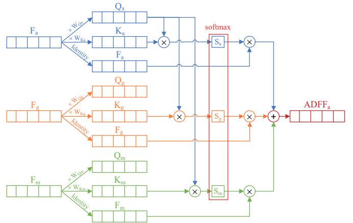
Fig. 6: Adaptive-weighted Sum for Accelerometer
