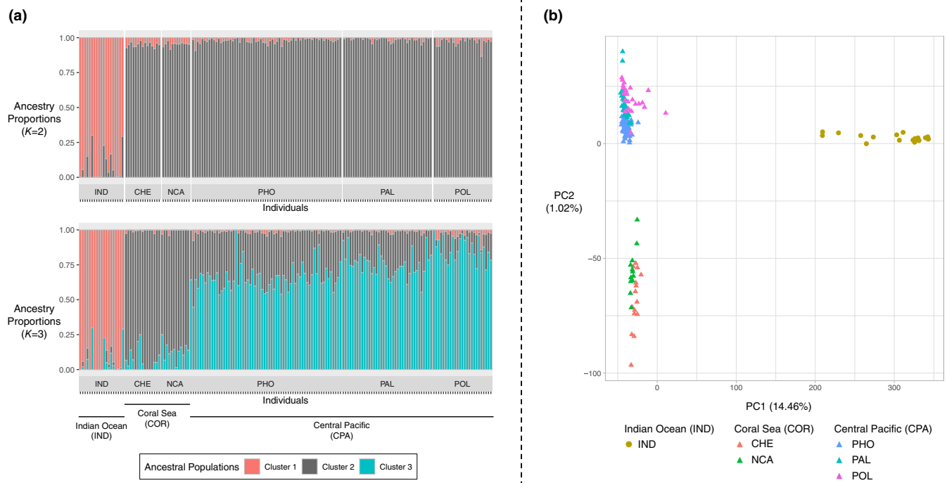
FIGURE 5 Individual-based population structure analyses. Ancestry proportions retrieved using the s SNMF algorithm with K = 2 and K = 3 ancestral populations (a) and principal component analysis (b)
