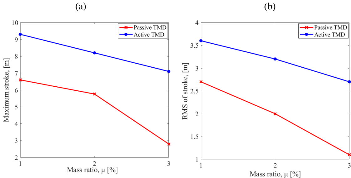
Figure 17: Passive TMD and ATMD stroke comparison under LC10 with different TMD mass ratios.
