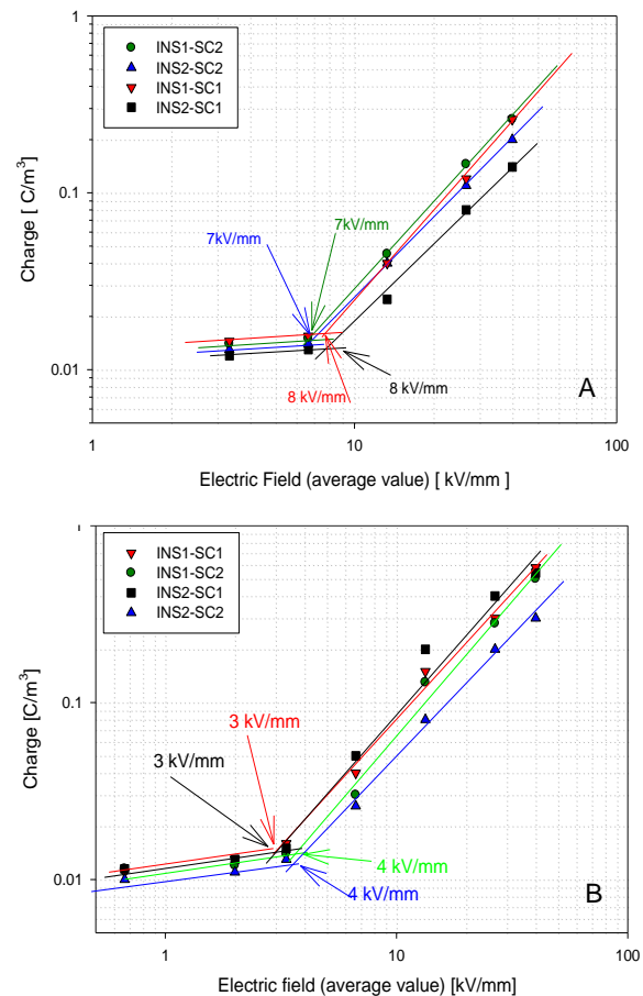
Figure 6: Space charge characteristics for mini-cables at 25°C (A) and 70 °C (B). The thresholds for space charge accumulation are indicated by arrows.
