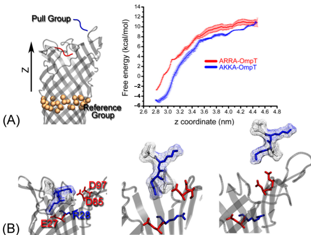
Figure 6. (A) The reference group and the pull group are used for umbrella sampling. The ligand backbone is shown as tube in red and blue, representing the initial and final positions of the ligand moving away from OmpT in the z-direction, shown next to the free energy landscape for binding of the ARRA and AKKA ligands to OmpT. (B) Three different snapshots were selected for umbrella sampling with the COM distance between the reference and pull groups being 2.8, 3.7, and 4.4 nm, respectively.
