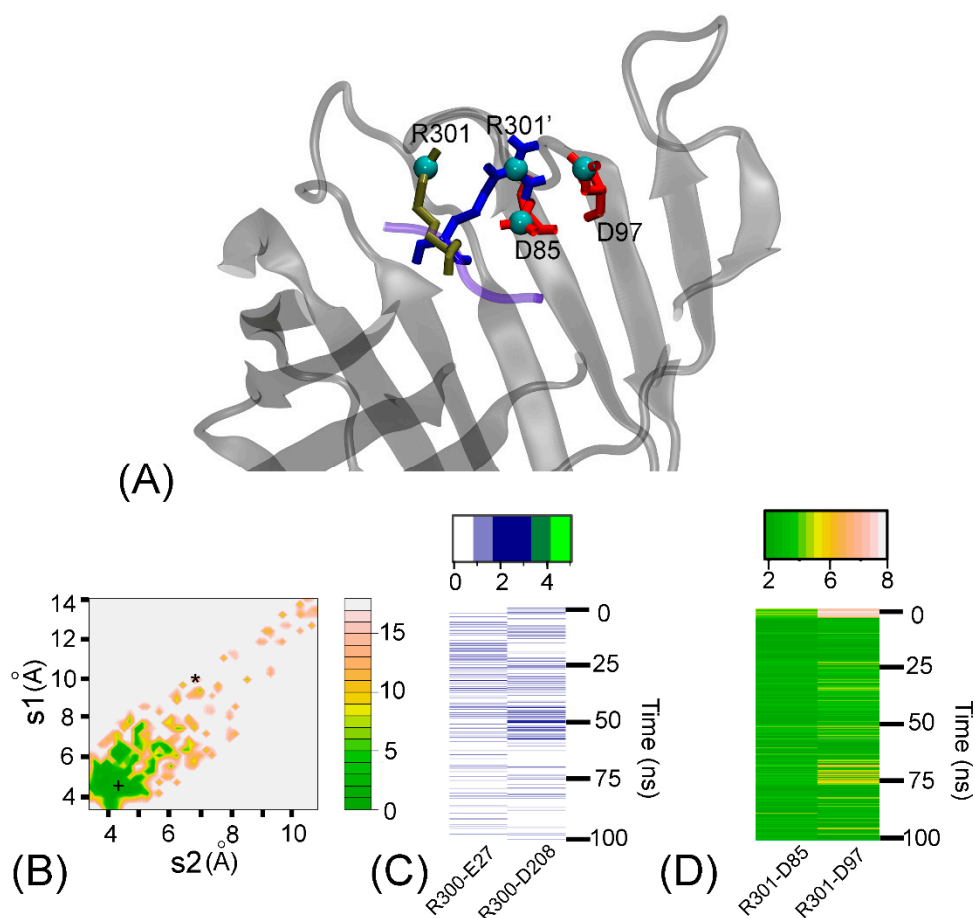
Figure 2. (A) Superposition of two conformations of the R301 residue of the ARRAs-OmpT complex at 0 ns (brown) and at 100 ns (blue). The neighboring residues D85 and D97 of OmpT are in close contact with R301 and are highlighted in red. (B) The two-dimensional free energy landscape as a function of distances s_1 and s_2 (defined in the text) for the 100 ns simulation. The asterisk (*) and cross (+) indicate the distances for the first and last simulation snapshots, respectively. (C) Time series of the number of hydrogen bonds between selected active site residues (E27 and D208) of OmpT and basic residue R300 of the ARRAs peptide. Hydrogen bonds were calculated with a donor-acceptor distance of 3.5 Å and an angle of 35° between donor-H-acceptor positions. (D) Time series of closest contact distances of salt bridges between selected active site residues (D97 and D85) of OmpT and basic residue R301 of the ARRAs peptide. The distance of salt bridges was calculated using the smallest native distance between two residues.
