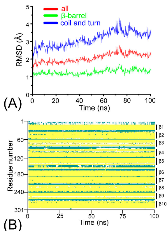
Figure A1. (A) Root mean square deviation (RMSD) of the ARRA-OmpT complex with respect to the initial structure for the carbon alpha atoms of all residues (red), the coil and turn structural elements (blue), and the \beta -barrel (green) during the 100 ns production simulation. (B) Temporal evolution of the secondary structure elements. The beta sheets, turns, and coil regions are shown in yellow, green, and white, respectively. Markers \beta 1 to \beta 10 represent the ten different beta sheets of OmpT.
