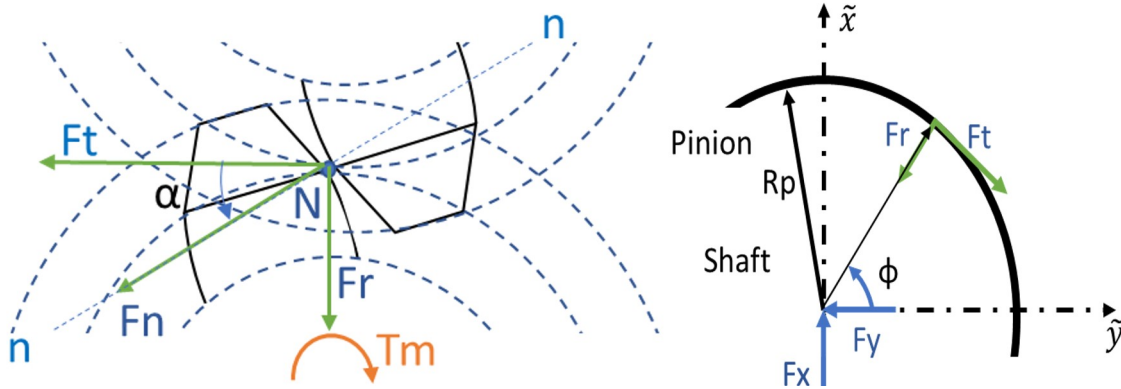
Figure 3: Gear simple model
