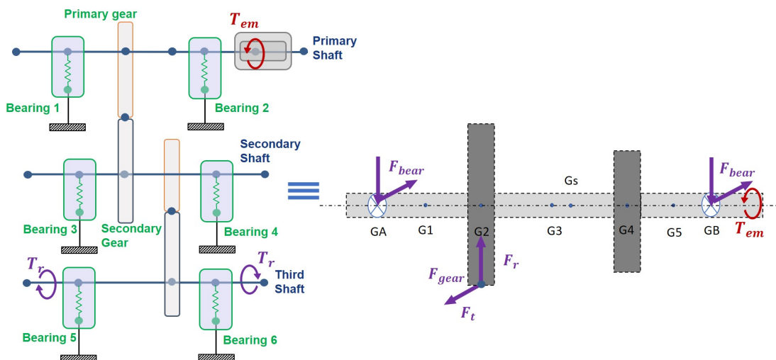
Figure 1: Rotor Bearing Model
