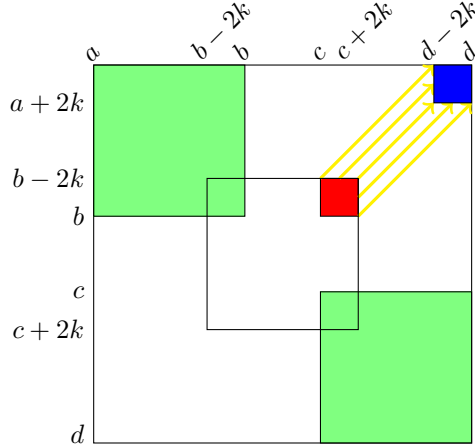
Figure 3: The submatrix of \mathcal{D} corresponding to a tall maximal trapezoid T = (a, b, c, d) . Green squares correspond to the values \mathcal{D}[i, j] with (i, j) \in [a \dots b]^2 \cup [c \dots d]^2 , for which the values are known. Except for the green squares, only the values in the red square, yellow diagonals, and the blue square can be smaller or equal to k . The processing of T must compute the values in the blue square given the values in the red square.
