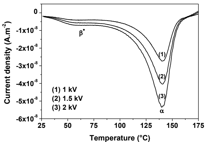
Fig. 2. TSDC profiles of PEN polarized at T_P = 130^\circ\text{C} : evolution of the \beta^* and \alpha peaks with the applied voltage V_P .
