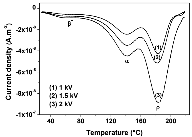
Fig. 3. TSDC profiles of PEN polarized at T_P = 170^\circ\text{C} : evolution of the \beta^* , \alpha and \rho peaks with the applied voltage V_P .
