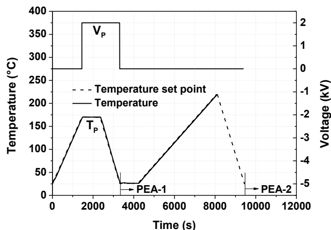
Fig. 1. Voltage and temperature protocol of TSDC measurements. Dotted and solid lines represent respectively the set point temperature and the measured temperature along the cycle.
