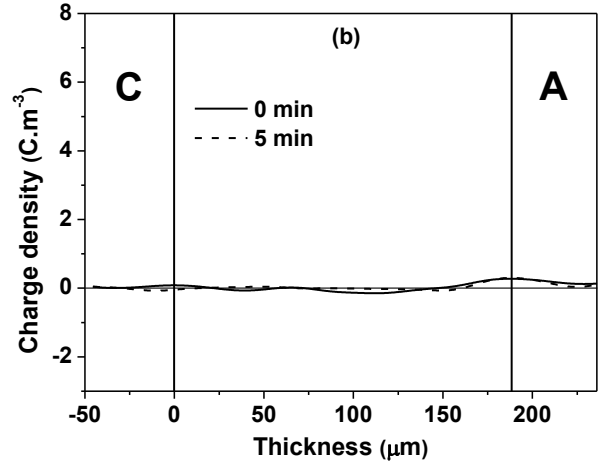
Fig. 5. Space charge profiles by PEA in Volt off for PEN previously polarized at 170°C: (a) Before reheating (PEA-1) of TSDC protocol; (b) After reheating (PEA-2) of TSDC protocol; C (Cathode), A (Anode).
