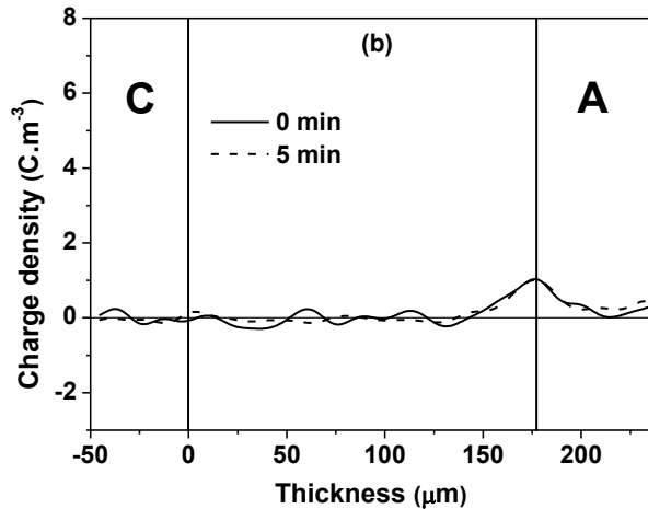
Fig. 4. Space charge profiles by PEA in Volt off for PEN previously polarized at 130°C: (a) Before reheating (PEA-1) of TSDC protocol; (b) After reheating (PEA-2) of TSDC protocol; C: Cathode, A: Anode during pre-polarization..
