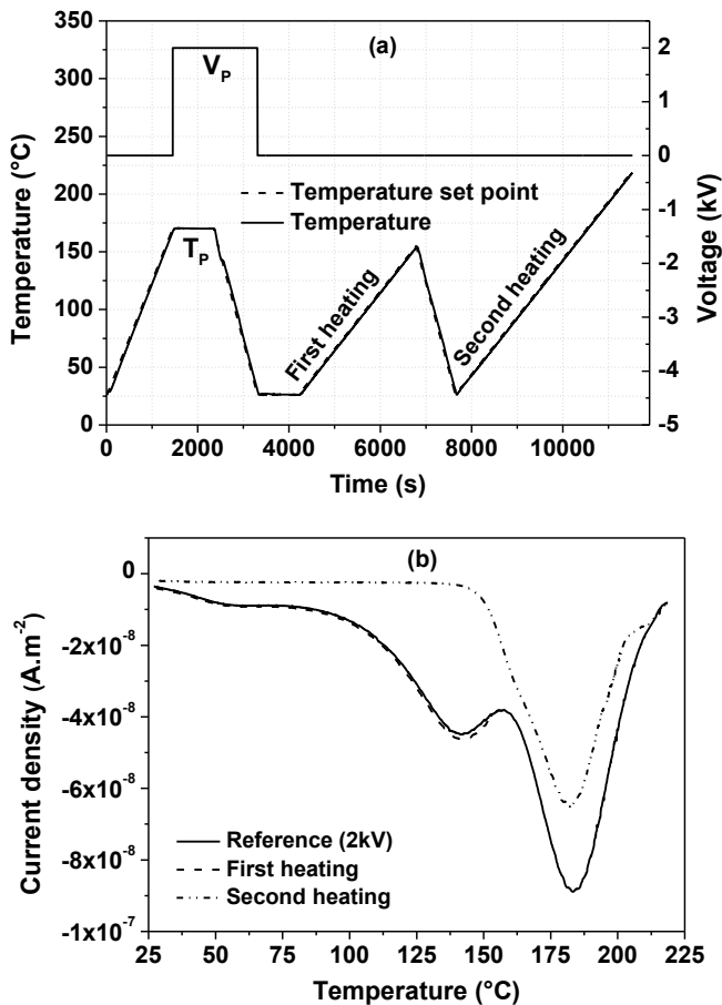
Fig. 6. (a) Voltage and temperature protocol for partial heating method; (b) TSDC responses without partial heating (solid line), after the first partial heating to 150°C (dashed line) and after the second heating rate (dash-dotted line).
