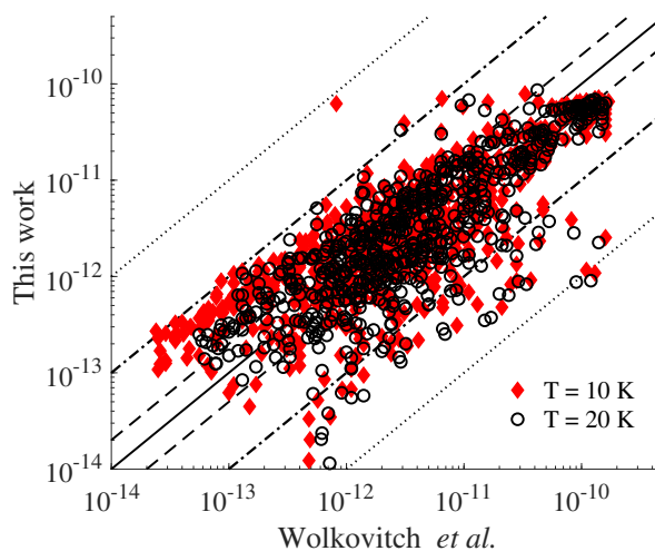
FIG. 7. Direct comparison of Wolkovitch et al. 25 CCS- H_2 fine-structure resolved rate coefficients and CCS-He ones provided in this work at 10 K (red diamonds) and 20 K (black open circles). The solid line represents a perfect agreement between the two sets of data; dashed, dashed-dotted and dotted lines delimit the regions where the rate coefficients differ by less than a factor of 2, 10 and 100, respectively.
