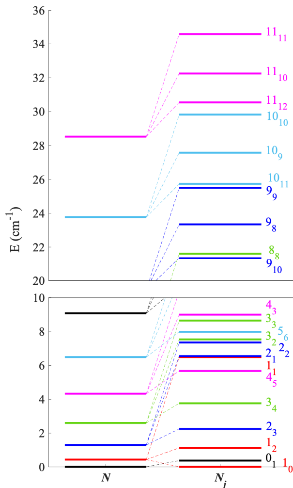
FIG. 2. Representation of the rotational (left) and fine structure (right) energy levels of the \text{CCS}(^3\Sigma^-) radical.
