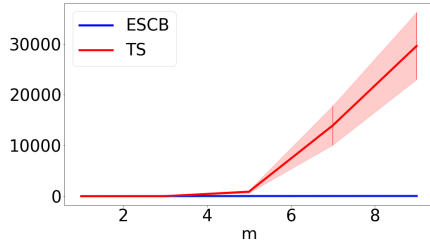
(a) \delta = 0.1 and T = 4.10^4 , Set of paths \mathcal{X}^p
