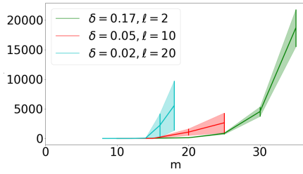
(a) Set of paths \mathcal{X}^p combinatorial set
