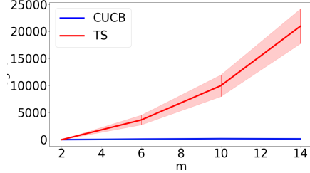
(b) \delta = 0.05 and T = 10^5 , set of matchings \mathcal{X}^m
