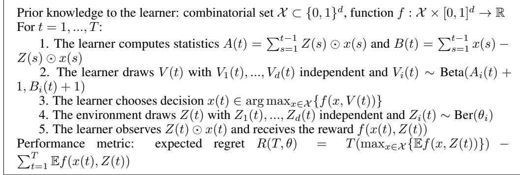
Figure 1: TS for combinatorial semi-bandits with Bernoulli rewards and uniform prior.
