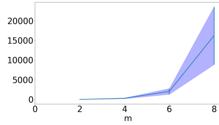
(b) Set of matchings \mathcal{X}^m combinatorial set \frac{\Delta}{m} = \frac{1}{100} and \ell = m
