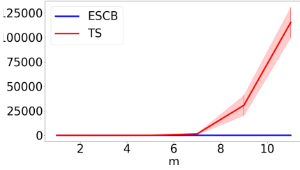
(a) \Delta = 1 and T = 4.10^5 , set of paths \mathcal{X}^p
