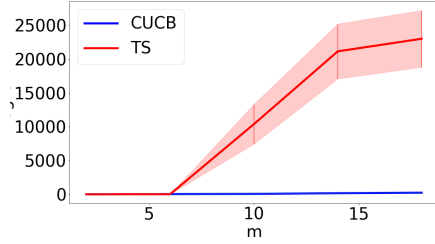
(b) \Delta = 1 and T = 10^5 , set of matchings \mathcal{X}^m
