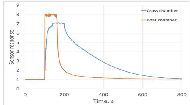
Figure 5. Experimental sensor response toward 50 ppm of ethanol in both chambers - injection during 1 min
