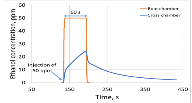
Figure 4. Ethanol concentration simulation in both chambers; injection at t=134\text{s} during 1 min
