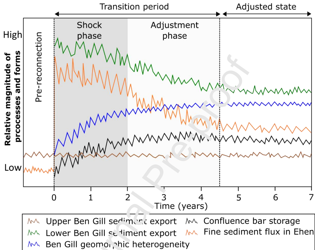
Figure 10: Conceptual representation of the relative magnitudes of processes and forms and their trajectories in Ben Gill, at the confluence and in the uppermost River Ehen over the study period. The point on the X-axis labelled 0 is October 2014, when Ben Gill was reconnected to the Ehen. All changes and trajectories displayed are derived from the evidence presented in Section 4. Lines highlight the general trends whilst stressing the occurrence of short term fluctuations caused by event-based and seasonal variability.
