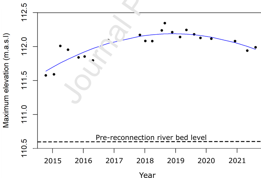
Figure 8: Maximum elevation of the confluence bar, measured from successive DEMs, from the first aerial survey in October 2014 to August 2021. The pre-reconnection riverbed level
