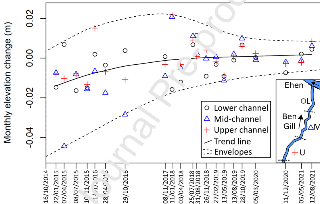
Figure 5: Mean monthly bed elevation changes for the lower, middle, and upper subsections of the Ben Gill channel. Each set of three points represent elevation changes from the previous survey (22/01/2015 points represent elevation changes from the first survey in October 2014). The map in the lower right indicates the locations of these subsections; arrows show flow direction. Data was fitted with a smooth spline regression trend line ( P < 0.05 , R^2 = 0.4 ).
