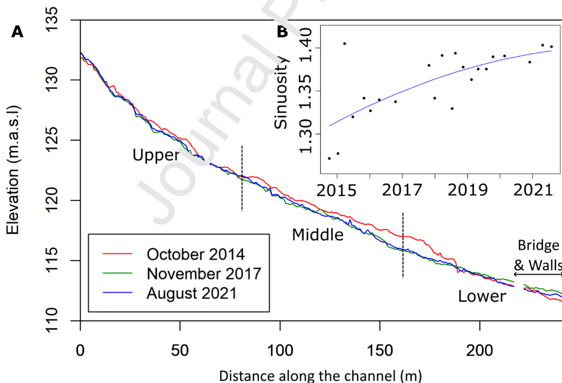
Figure 6: A : Channel bed elevations in Ben Gill derived from 243 fixed points, one every metre within the active channel, extracted from DEMs. The gap at 220 - 226 m is where an
