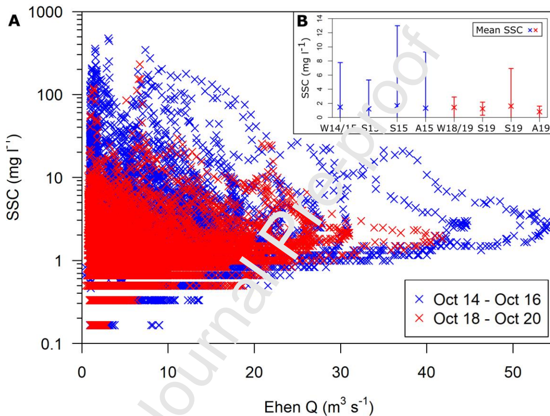
Figure 9: A: Suspended sediment values plotted against discharge for the upper River Ehen at Bleach Green, situated 550 m downstream of the confluence. Blue crosses represent values during the first two years of the reconnection while red crosses represent SSC values 4 - 6 yr after the reconnection. B: Comparison of seasonal mean and standard deviation SSC values for the 2014 - 2015 and 2018 - 2019 seasons; W = Winter, S = spring, S = Summer, A = Autumn, using Northern Hemisphere meteorological seasons.
