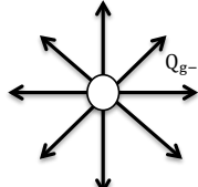
Fig. 4.2. Field line of Q_{g-}
