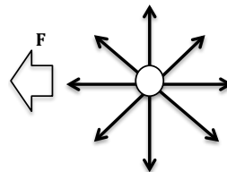
Fig. 4.5: repel each other
