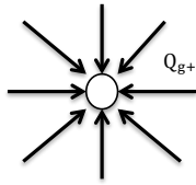
Fig. 4.1. Field line of Q_{g+}
