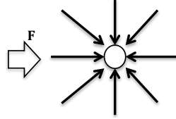
Fig. 4.3: two positive g-charges are attractive to each other
