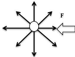
Fig. 4.4: attractive to each other
