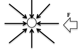
Fig. 4.3: two positive g-charges are attractive to each other
