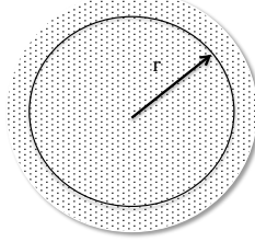
Fig. 4.6: Accelerating Expansion of Universe
