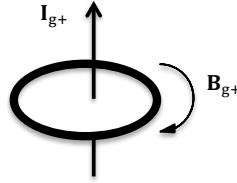
Figure. 4.7: “The left-hand rule” for gravito-magnetic field \mathbf{B}_{g+}
