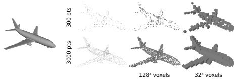
Fig. 2: Visualization of voxelizations at resolutions 32^3 and 128^3 of input point clouds with 300 and 3000 points.
