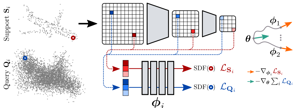
Fig. 1: Overview of our method. Our input is a sparse point cloud (Support S_i ) and our output is an implicit neural SDF f . f is a neural network comprised of a convolutional encoder (top in gray) and an MLP decoder (bottom in gray). The decoder predicts SDF values for 3D points (red/blue circles) through their spatially sampled features (squares in shades of red/blue) from the encoder’s activation maps. Following a gradient-based few-shot learning algorithm (MAML [21]), we learn a meta-decoder in encoder feature space, parameterized with \theta , that can quickly adapt to a new shape, i.e. new parameters \phi_i , given its support. This is achieved by iterating per-shape 5-step adaptation gradient descent (orange arrow) using the support loss \mathcal{L}_{S_i} , and one-step meta gradient-descent (green arrow) by back-propagating the Query set ( Q_i ) loss \mathcal{L}_{Q_i} evaluated with the specialized parameters \phi_i w.r.t. the meta-parameters \theta . At test time, 5 fine-tuning iterations are performed similarly starting from the converged meta-model to evaluate f .
