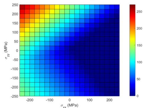
Figure 1 : Evolution of the predicted normalized H_{95}: H at M = 0.95 \times M_{sat} , under biaxial stress states. The magnetic excitation and the magnetic sensors are along x (RD).
