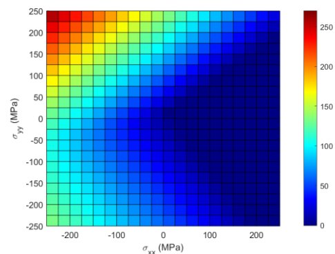
Figure 1 : Evolution of the predicted normalized H_{95}: H at M = 0.95 \times M_{sat} , under biaxial stress states. The magnetic excitation and the magnetic sensors are along x (RD).
