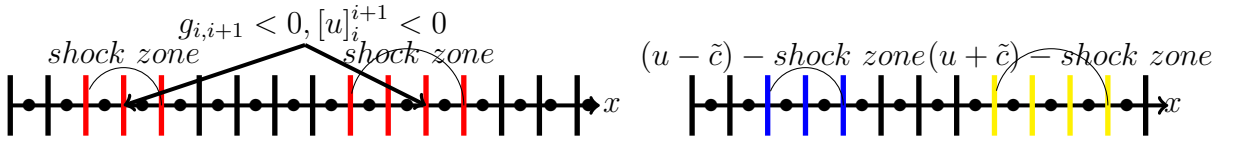
Figure 4: Two different steps of the shock detector. Step 1 (left) shock zone detection, step 2 (right) (u - \tilde{c}) -shock or (u + \tilde{c}) -shock identification. Interface colors: shock zone (red), 1-shock (blue), 3-shock (yellow) and for other waves types (black)
