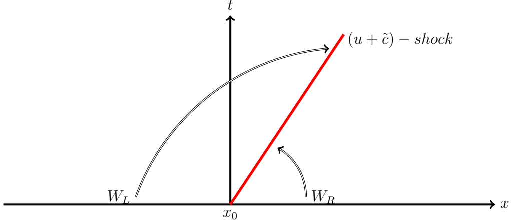
Figure 8: The exact solution of the Riemann problem for the test 2.
