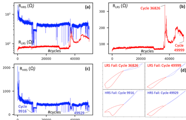
Fig. 6. (a) R_{LRS}/R_{HRS} resistances in log scale. (b) R_{LRS} in linear scale. (c) R_{HRS} in linear scale. (d) I-V characteristics extraction for specific cycles.
