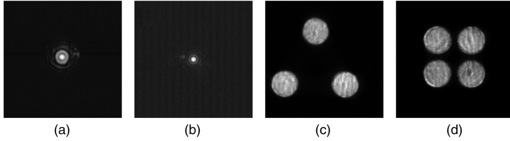
Fig. 10 Signals from CACTI in response to the optimized flat wavefront. (a) The PSF on the science camera. (b) The optimized PSF on the focal plane of the PWFS tips. (c) The 3PWFS pupils on Camzyra at 5\lambda/D modulation. (d) The 4PWFS pupils on Cam4p at 5\lambda/D modulation.
