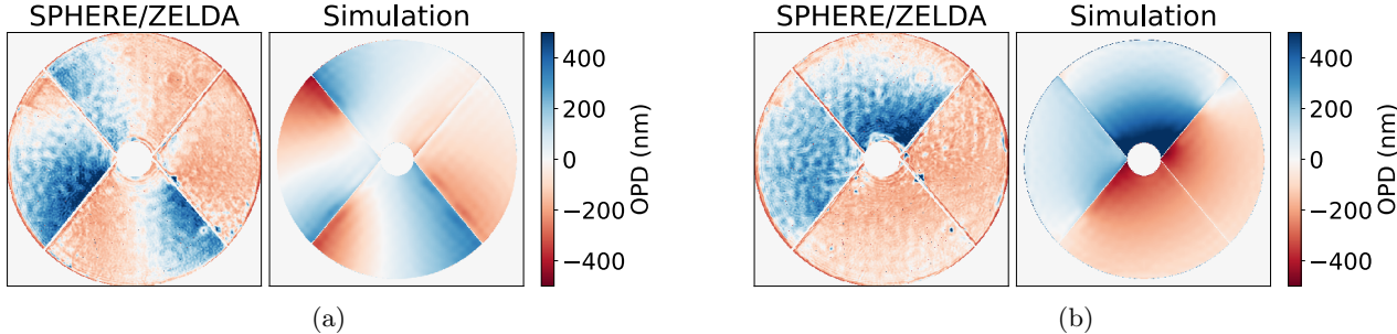
Figure 9: Qualitative reproduction of the LWE post-AO residuals observed on SPHERE with the ZELDA sensor.
