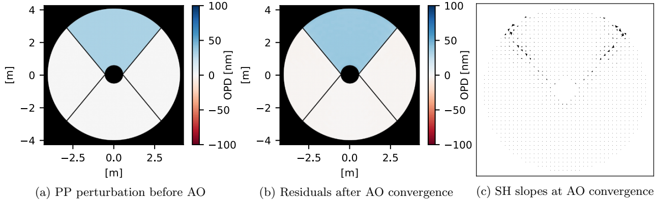
(a) PP perturbation before AO (b) Residuals after AO convergence (c) SH slopes at AO convergence Figure 6: AO response to a petal-piston of 32 nm peak-to-valley amplitude (weak-phase regime) as perturbation. (a) perturbation before AO, the OPD is 21 nm rms. (b) post-AO residuals after convergence, the OPD rms is 24 nm rms. (c) SH slopes at convergence.
