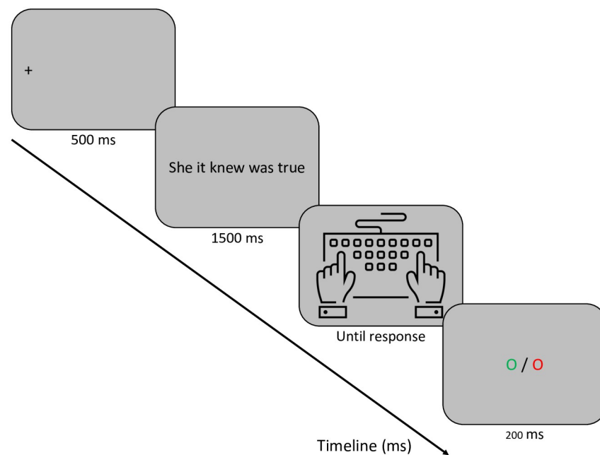
Fig 7. Schematic of one experimental trial for the parallel presentation procedure of Experiment 3. As in the previous experiments, responses were given via the left and right arrow keys of the keyboard.
