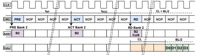
Fig. 8: Precharge to Read commands transition time
