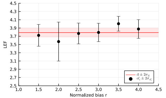
Figure 5: Measured values of the LEF as a function of the normalized bias current r .
