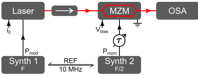
Figure 1: Experimental setup.
