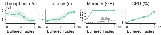
Figure 13: Effect of the buffer size B on SYN.
