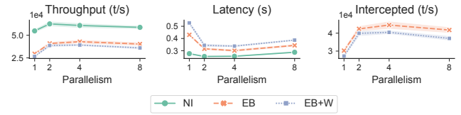
Figure 14: Scalability of MOV query.
