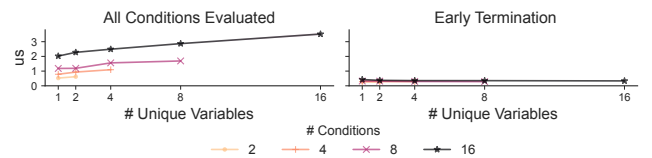
Figure 11: Time to run a single evaluation of the predicate.
