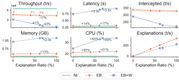
Figure 7: Performance impact of explanations for SGA.
