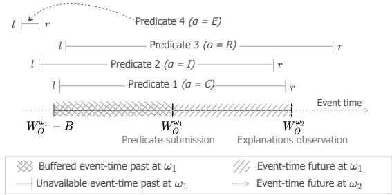
Figure 2: Examples of the four possible explanation markers for an operator O and predicates with different time intervals.
