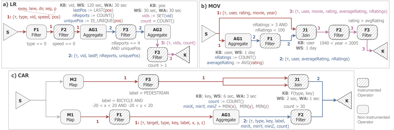
Figure 5: Queries used in the evaluation (along with SGA, presented in Figure 1).
