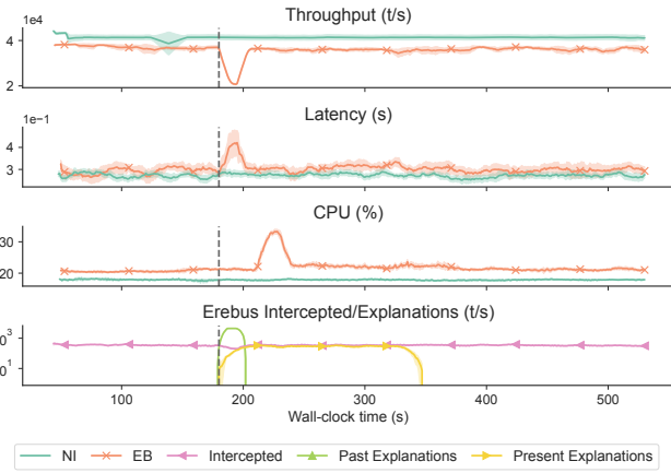
Figure 6: Performance of SGA over time.
