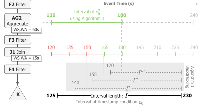
Figure 3: Timestamp translation for an operator path of the query presented in Figure 1.
