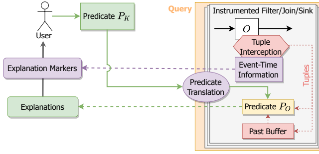
Figure 4: High-level architecture of Erebus .
