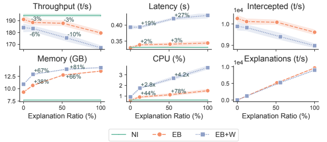
Figure 10: Performance impact of explanations for CAR.
