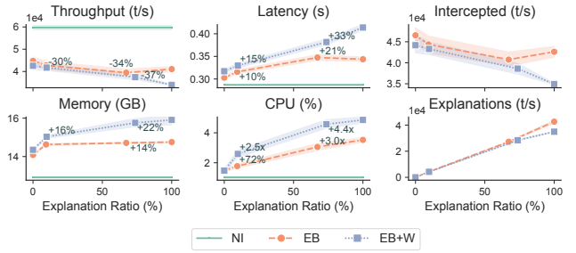
Figure 9: Performance impact of explanations for MOV.
