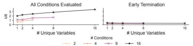
Figure 11: Time to run a single evaluation of the predicate.
