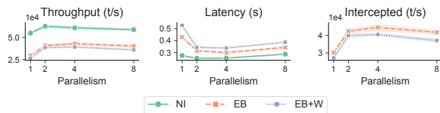
Figure 14: Scalability of MOV query.
