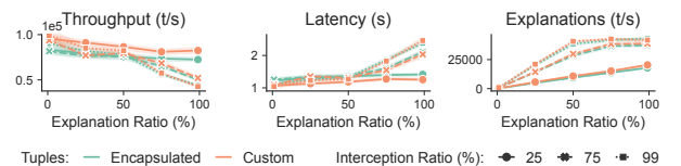
Figure 12: Effect of Erebus ' overheads i_O , e_{P_O} , D on SYN.
