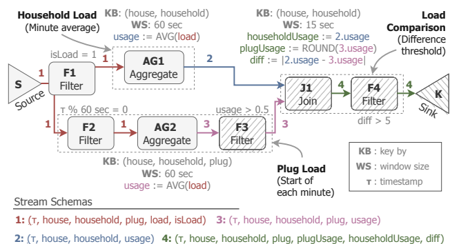
Figure 1: Example streaming query from Erebus ' evaluation.
