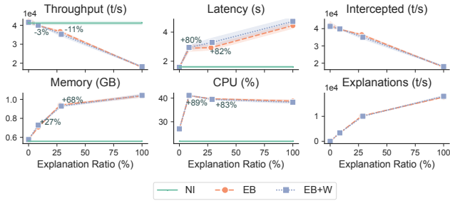
Figure 8: Performance impact of explanations for LR.
