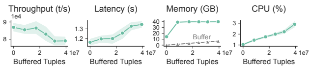
Figure 13: Effect of the buffer size B on SYN.
