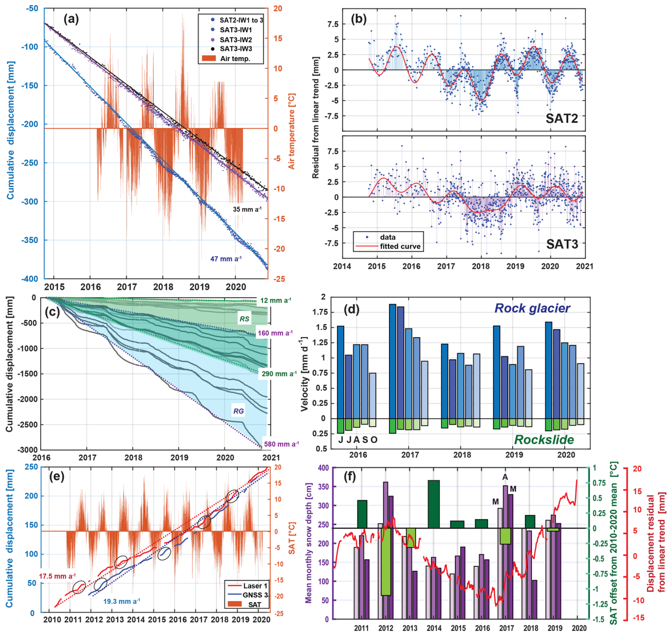
Figure 5. Displacement measurements at Gámanjunni-3 (a–d) and Mannen (e, f). (a) Cumulative displacement rates from the three satellite corner reflectors on Gámanjunni-3, showing average annual displacement rates between 35 and 47 mm a -1 along satellite radar LOS. (b) Residuals from the linear trend for SAT2 (upper) and SAT3 (lower). We fitted a third-order sinusoidal curve (red line) to the residual points. The fit indicates annual variation and a trend towards negative residuals until 2018. (c) Cumulative displacement along GB radar LOS derived at a total of 18 points dispersed over the rockslide (RS) and rock glacier (RG) area (Fig. 1) based on GB InSAR. The green shaded envelope shows the RS points, and the light blue envelope indicates the RG points. Velocities between 10 and close to 600 mm a -1 are encountered. (d) Average daily displacement averaged over a month along GB radar LOS for one GB InSAR point at the rock glacier (blue bars) and a point at the rockslide area (green bars). For each year the months between June and October are shown. The graph shows the highest velocities early in the melting season and the highest absolute velocities in 2017. (e) Mannen: cumulative displacement rates for GNSS3 and Laser1, plotted with SAT since 2010. There are obvious acceleration phases (some indicated by ellipses) during early summer (May–June). (f) Residuals from the linear trend for Mannen Laser1 (red line) against MAAT deviation between 2010 and 2020 (green bars) as well as snow depth (purple bars) for the months March through May. There is a clear decrease in displacement rates between 2013 and 2017, which seems to be related to higher air temperatures and lower snow coverage.
