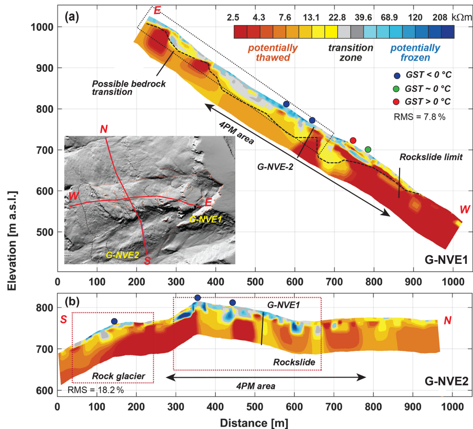
Figure 8. The long ERT profiles for Gámanjinni-3. The colour scale follows the laboratory analysis shown in Fig. 3 and is a logarithmic scale. (a) G-NVE1, showing high-resistivity layers down to ca. 700 m a.s.l. (box). The dashed line indicates the possible transition to solid bedrock. (b) G-NVE2, the cross-profile over the rock glacier and the lower rockslide area, indicated by the red boxes. The circles in both profiles indicate the location and mean annual GST in the vicinity of the profiles based on Eriksen (2018) and subsequent measurements (Gudrun D. Majala, NVE, unpublished data, 2020). They show sub-zero temperatures in areas with high-resistivity surface layers and higher values below 700 m a.s.l. The part of the profile used for the four-phase model (4PM) is indicated in both profiles (Fig. 11).
