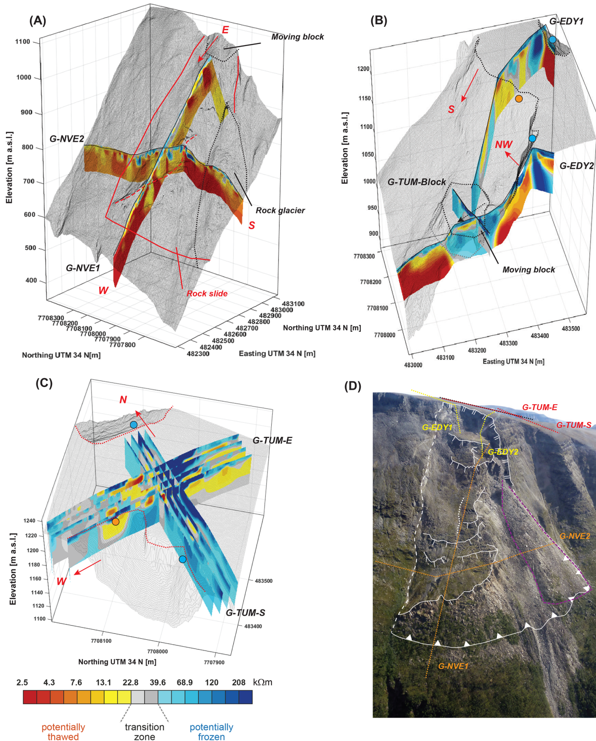
Figure B1. 3D plots showing the ERT profiles in relation to topography for Gámanjunni-3. (a) G-NVE1 and G-NVE2. The rockslide (red) and rock glacier (black) are delineated. The black stippled line indicates the lower limit of the moving block. (b) The rock wall profiles G-EDY1 and G-EDY2 and the ERT profile over the moving block (G-TUM block). The moving block is indicated by the black line, as is the crest between the rock wall and top plateau. The circles show the location of the rock wall loggers (orange: >0^{\circ}\text{C} in annual average, blue: <0^{\circ}\text{C} ). (c) Quasi-3D profiles on the plateau (G-TUM-S and E). The red line shows the crest, with the circles like in (b). (d) Oblique image of the instability at Gámanjunni-3 as in Fig. 2a. The approximate location of the ERT profiles is drawn on the images. © NGU.
