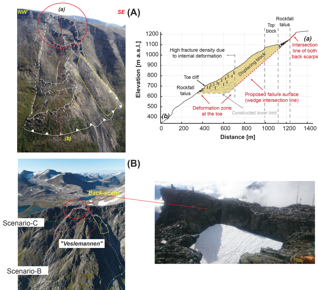
Figure 2. (A) Image (left, © NGU) and structural–geological model (right) of Gámanjunni-3 (Böhme et al., 2016, 2019). The yellow stippled line outlines the rock glacier, and the red circles show the back scarp and the moving block. The white lines indicate the different parts of the rockslide (scarps, lateral border, slide front) mapped by Eriksen et al. (2017); similar mapping is also shown in Fig. 1b by NGU. The geological model forms the basis for the stratigraphy used for thermal modelling (Figs. 7 and A1, 2). (B) Overview image of the Mannen instability (© I. Skrede/NVE) and close-up image of the back scarp. The red line shows the moving part of the slope according to scenario C. The red circle shows the back scarp and the deep fracture below, which in this picture is still snow-covered. The stippled yellow line indicates the recently failed Veslemannen (Kristensen et al., 2021).
