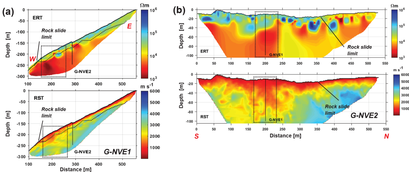
Figure C1. Resistivity and seismic velocities for the 4PM at Gámanjunni-3 for (a) G-NVE1 and (b) G-NVE2. Note that the profiles are subsets of G-NVE1 and G-NVE2 and are thus shorter than shown in Figs. 8 and B1. Note also that the colours for the electrical resistivity do not correspond to the colour scale derived from the laboratory analysis (Fig. 3) but are the original results first presented in Hauck and Hilbich (2018). The possible fracture zones mentioned in the paper are indicated as a box, while the possible lower permafrost limit is drawn as a line in (a).
