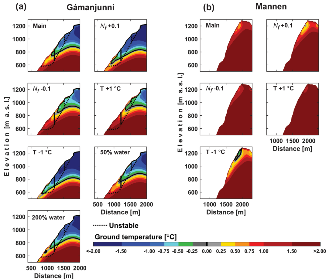
Figure A2. Sensitivity plots for the modelled ground thermal regime of (a) Gámanjunni-3 and (b) Mannen. The main run is the presented run in Fig. 7, and the panels show modelled ground temperature in response to changes in N_f factor ( N_f 0.1 means that N_f is increased by 0.1; N_f - 0.1 means that N_f is decreased by 0.1), forcing SAT ( T+1\text{ °C} means that SAT is increased by 1\text{ °C} ; T-1\text{ °C} means that SAT is decreased by 1\text{ °C} ) and water content in the subsurface (50 % water means that water content is halved and the remaining fraction is added to the mineral fraction; 200 % water means that water content is doubled by reducing the mineral fraction). GT and permafrost geometry change in response to these variations. It is noteworthy at Mannen that only small changes in snow or forcing temperatures would produce considerably more permafrost in the unstable area. Due to limited assumed sediment cover for the Mannen site, we did no sensitivity plot for the water content in bedrock, which is low.
