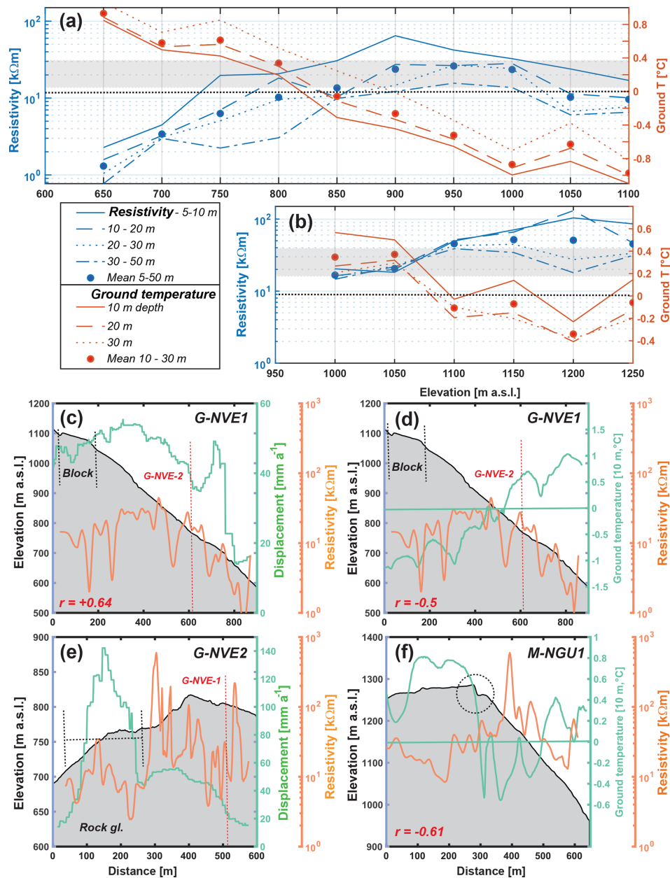
Figure 13. Relationship between resistivity, modelled ground temperature (GT) and rockslide displacement rates along selected profiles for Gámanjinni-3 and Mannen, binned in 50 m intervals. At Mannen, poorer InSAR coverage restricted the analysis of the velocity–ERT relationship. The black dotted line indicates the modelled 0 °C line, while the grey area indicates the electrical resistivity transition resolved from laboratory analysis (Fig. 3). (a) Relationship between modelled ground temperature in three depths and extracted electrical resistivity for four different depth areas for G-NVE1. The solid circles display averages over all depths. The graph confirms the transition area for permafrost around 800 m a.s.l. (b) The same as (a) , but for Mannen (M-NGU). Here there is also a higher resistivity with lower temperatures, but the relationship is less clear. According to the modelling permafrost can be expected above 1100 m a.s.l. (c) Relationship between elevation, displacement rates and electrical resistivity for G-NVE1. ERT and displacement rates co-vary, with a significant correlation of r = 0.64 . The red line shows the crossing point for G-NVE2. (d) G-NVE1. Relationship between elevation, modelled GT and electrical resistivity. We observe a negative relation between GT and resistivity ( r = -0.5 ). The red line shows the crossing point for G-NVE2. (e) Cross-profile G-NVE2 over the rock glacier (dotted line) and rockslide area at ca. 700 m a.s.l. Resistivity is lower and displacement rates are much higher on the rock glacier than on the rockslide part, indicating different modes of movement (see main text). The red line shows the crossing point for G-NVE1. (f) M-NGU. Relationship between surface altitude, modelled GT and resistivity. We observe a negative relationship between GT and resistivity ( r = -0.61 ), with lower GT and higher resistivity values along the upper part of the steep slope. The location of the back scarp of the unstable area is indicated with a circle.
