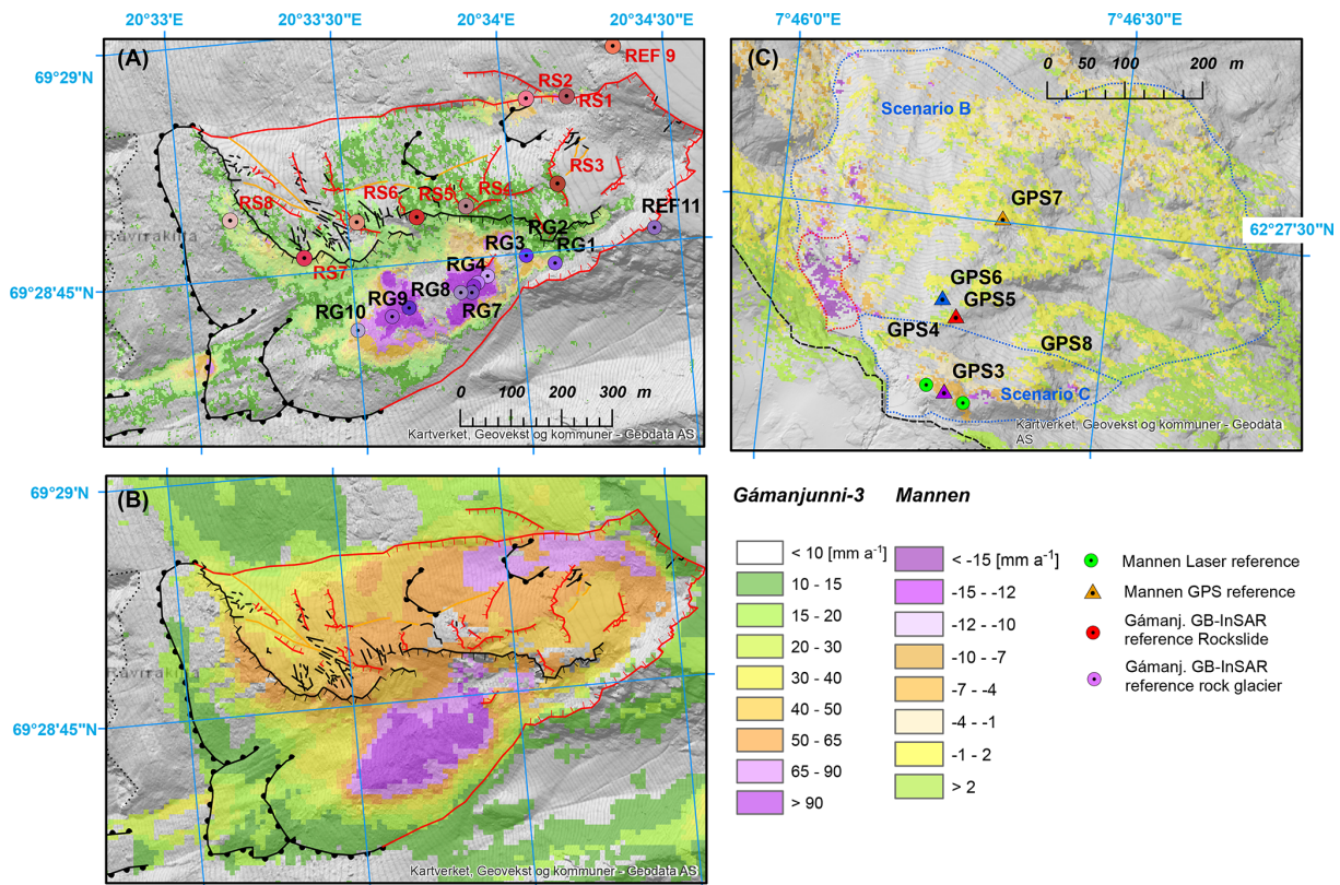
Figure 6. Spatial distribution of displacement rates for Gámanjinni-3 (a, b) and Mannen (c). (a) The GB InSAR map is an average for the summer 2020. The circles indicate the position of time series sampling shown in Fig. 5 on the rockslide (red) and the rock glacier (violet). The colour depth indicates relative differences in velocity. (b) Satellite 2D InSAR-derived averaged summer displacement rates collected between 2009 and 2014 using TerraSAR-X (Eriksen et al., 2017). Both show clearly higher velocities in the rock glacier area. (c) GB InSAR displacement rates along GB radar LOS of the Mannen instability from summer 2020, showing relatively low displacement rates outside the upper scar area. The recently failed rockslide Veslemannen (Kristensen et al., 2021) is delineated by the dotted red line. The dashed black line indicates the upper scarp area. The failure scenarios are based on Dahle et al. (2008). Note the different velocity scales for Gámanjinni-3 and Mannen. All base maps from © Statens Kartverk.
