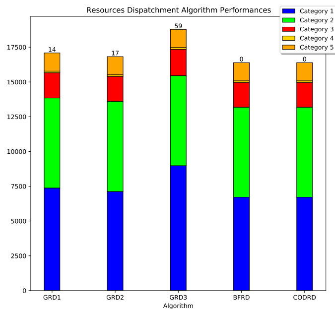
FIGURE 6: Objective Score performances for the different resources dispatch algorithms
