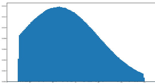
FIGURE 3: Truncated normal distribution with \mu = 45 , a = 10 , b = 120 and \sigma = 35
