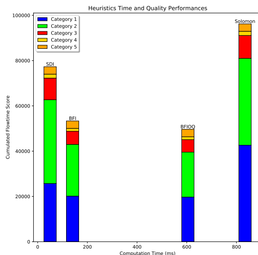
FIGURE 4: Graphic comparing computation time and cumulative objective score performances of the heuristics
