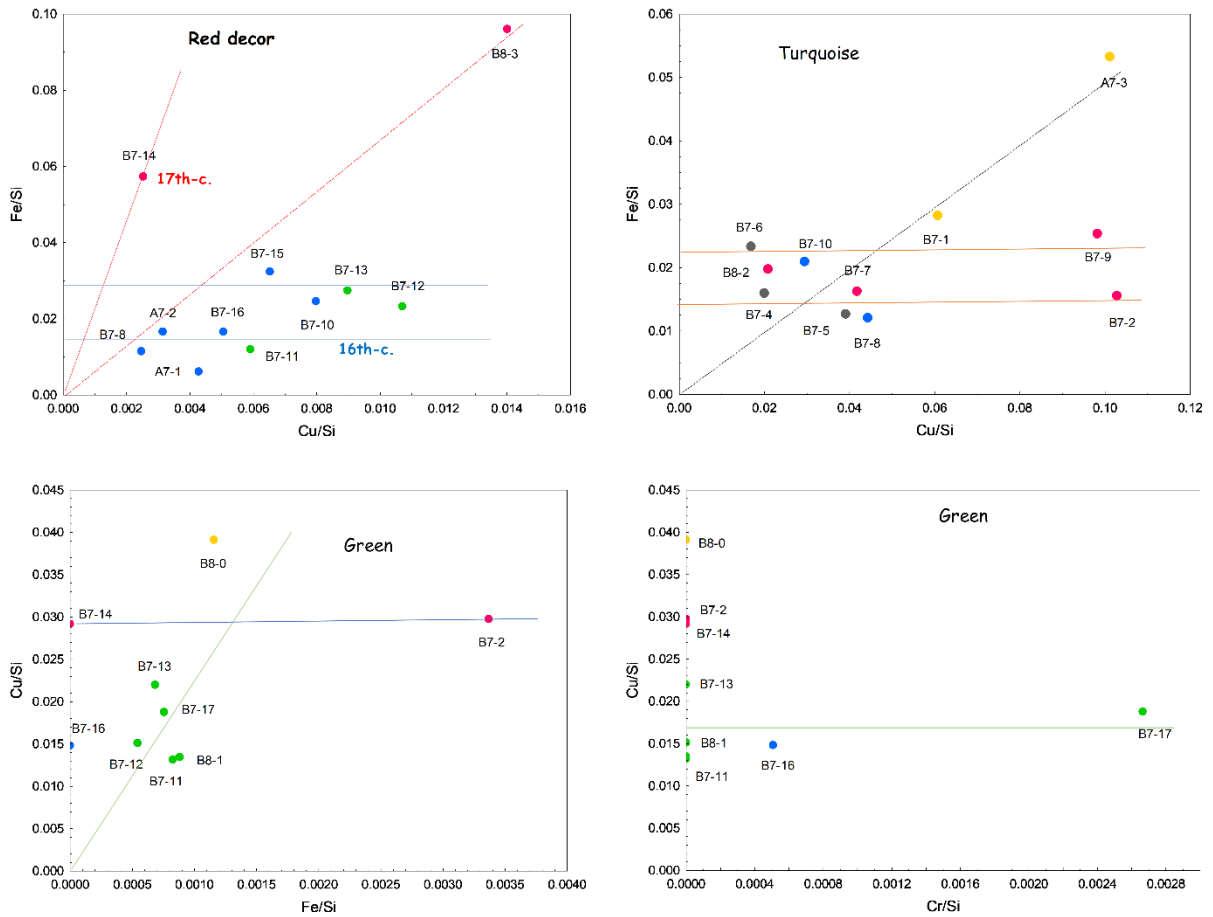
Fig. S7: Scatter plots of the weight % ratios of Fe/Si versus Cu/Si measured on red (upper left) and turquoise areas (upper right); Cu/Si versus Fe/Si (bottom left) and Cu/Si versus Cr/Si (bottom right) on green areas; see previous figures for symbols. Lines are guide for eyes.
