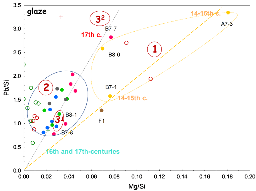
Fig. 3: Scatter plots of the weight % ratios of Sn/Si versus Pb/Si (upper) and Pb/Si versus Mg/Si (bottom) in the transparent glaze, see previous figures for symbols. Lines are guide for eyes.
